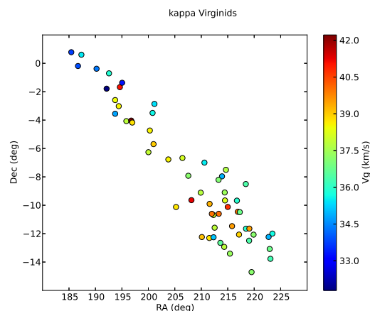
Figure 1 – Radiant plot of \kappa Virginids.
