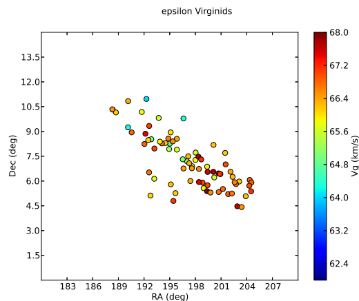
Figure 5 – Radiant plot of \epsilon Virginids.
