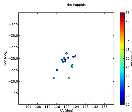
Figure 4 – Radiant plot of \rho Puppids.
