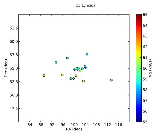
Figure 3 – Radiant plot of 15 Lyncids.
