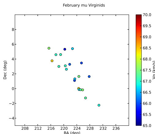
Figure 7 – Radiant plot of February \mu Virginids.
