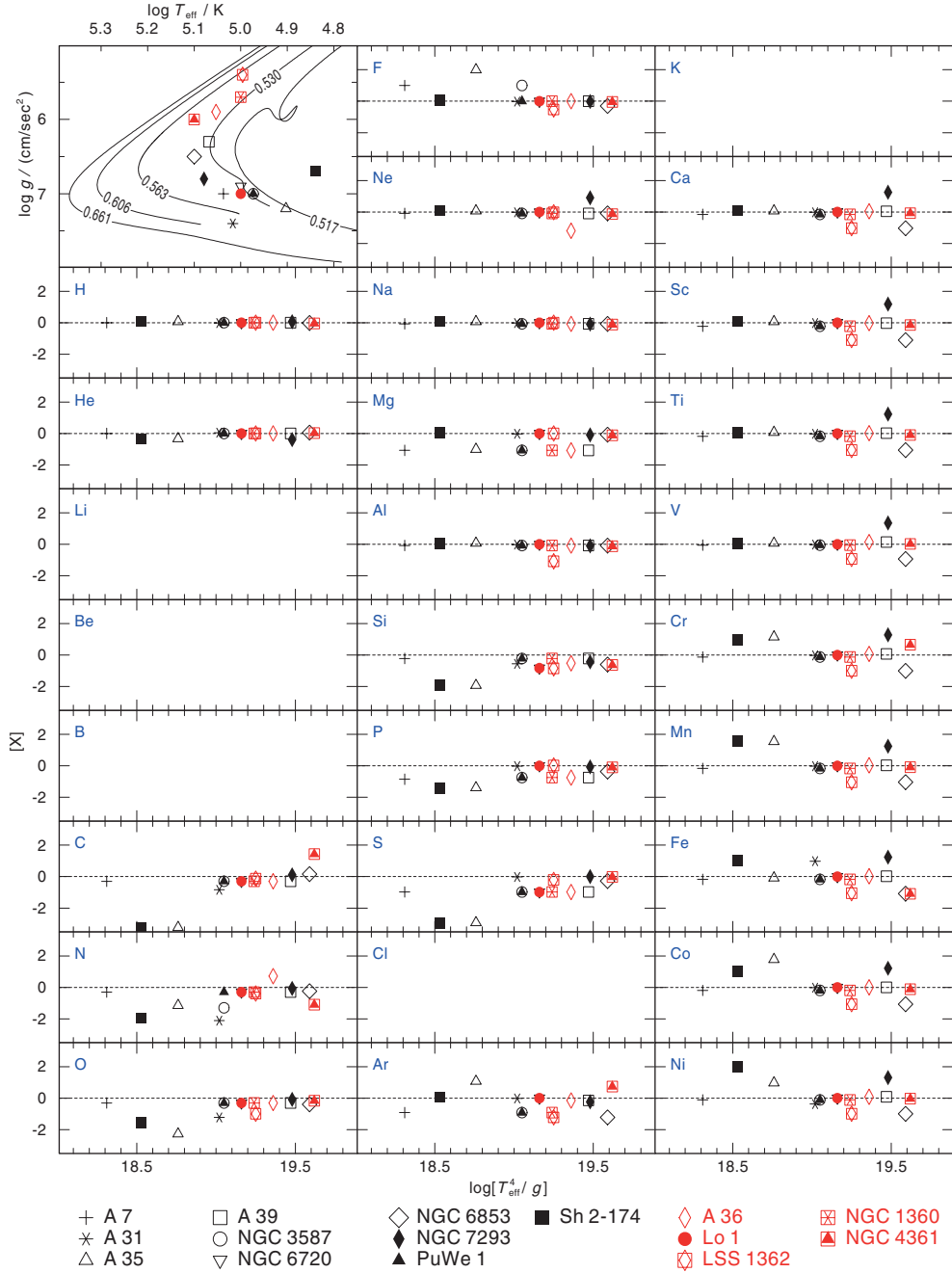
Figure 1. \log T_{\text{eff}} - \log g diagram (upper left) and chemical abundances as a function of \log [T_{\text{eff}}^4 / g] . DAO-type CS are displayed in black, O(H) types in red. The evolutionary tracks from Miller Bertolami (priv. comm.) are labeled with the stellar masses (in M_{\odot} ). [X] denotes \log(\text{abundance}/\text{solar abundance}) for species X.
