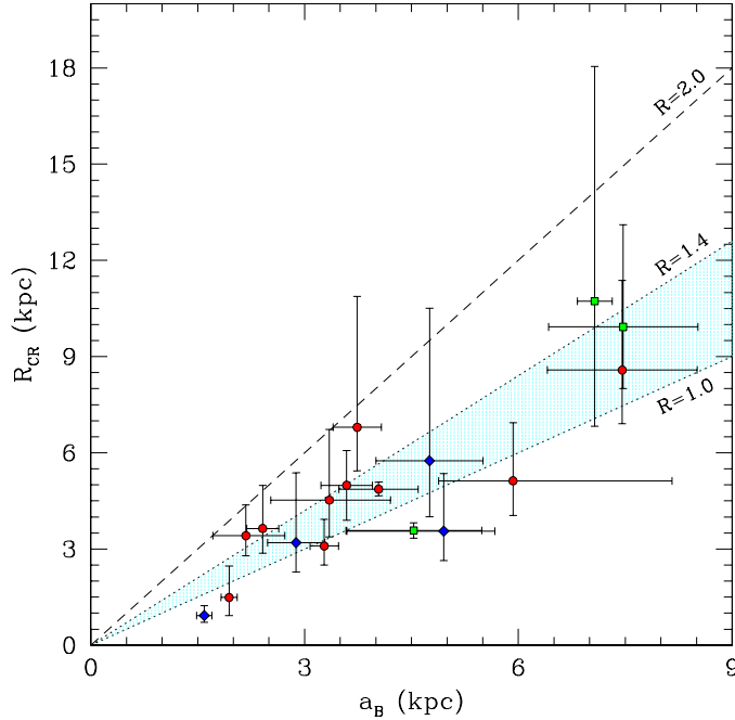
Fig. 1. The corotation radius R_{\text{CR}} as a function of the bar length a_{\text{bar}} for the barred galaxies with \Omega_{\text{bar}} measured by applying the stellar-based TW method. Red circles denote measurements for SB0 galaxies, blue diamonds correspond to SB0/a galaxies, and green squares represent spiral barred galaxies. The dotted lines correspond to \mathcal{R} = 1 and \mathcal{R} = 1.4 , respectively. They separate the forbidden ( \mathcal{R} < 1 ), fast-bar ( 1.0 \leq \mathcal{R} \leq 1.4 , hatched area), and slow-bar ( \mathcal{R} > 1.4 ) regimes. The dashed line marks \mathcal{R} = 2 .
