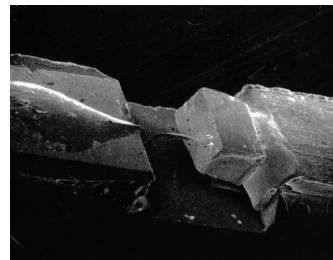
Figure 7: Electron micrograph of a Schottky junction used in millimetre receivers in the mid-70s; a whisker touches a gallium arsenide crystal (courtesy: Laboratoire de Physique, École Normale Supérieure).
