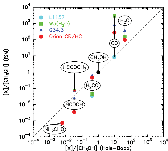
Figure 6. Molecular abundances in comet Hale-Bopp (CHO-bearing species) compared to those in the bipolar flow L1157 and several hot molecular core. From Bockelée-Morvan et al. (2000).
