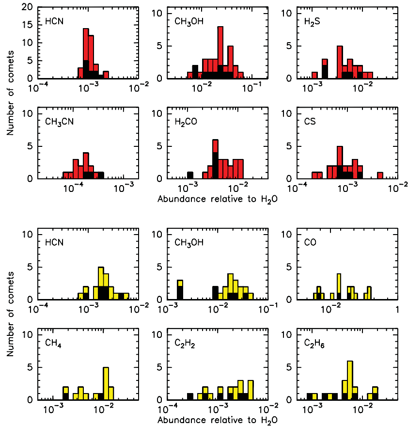
Figure 2. Histogram of molecular abundances relative to water from radio observations (top, Crovisier et al. 2009) and IR observations (bottom). The histogram for Jupiter family comets is in black.
