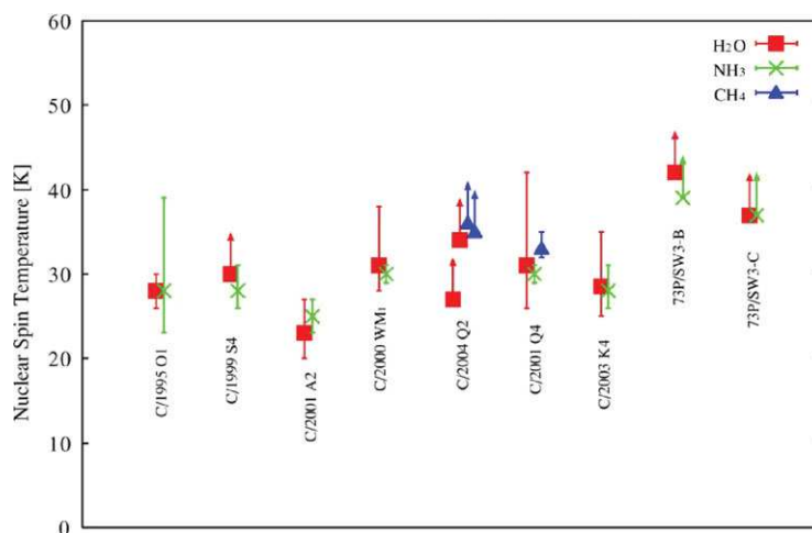
Figure 5. Comparison of nuclear spin temperatures of H 2 O, NH 3 and CH 4 observed in comets. From Shinnaka et al. (2011).
