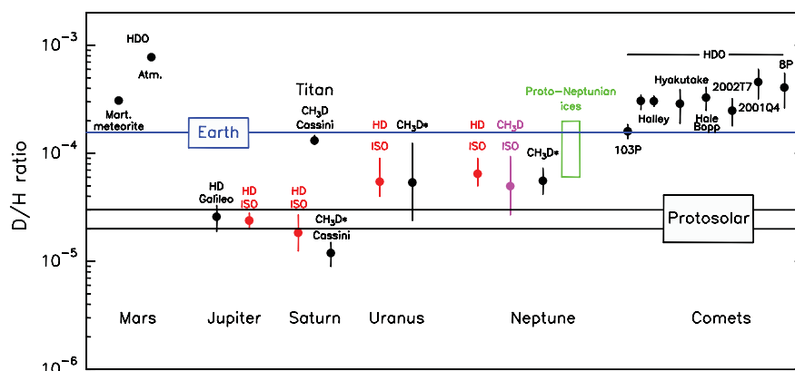
Figure 3. D/H in the Solar System.
