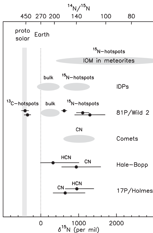
Figure 4. N isotope measurements in primitive matter of the Solar System, given either as ^{14}\text{N}/^{15}\text{N} ratios or \delta^{15}\text{N} values ( \delta^{15}\text{N} = (^{14}\text{N}/^{15}\text{N}) / (^{14}\text{N}/^{15}\text{N})_{\text{Earth}} - 1 ). Shown are the protosolar value measured by the Genesis mission (Marty et al. 2011), values for comet 17P/Holmes (Bockelée-Morvan et al. 2008), comet Hale-Bopp (Arpigny et al. 2003; Bockelée-Morvan et al. 2008) and other comets (Jehin et al. 2009), dust particles of comet 81P/Wild 2 collected by the Stardust mission (McKeegan et al. 2006), interplanetary dust particles IDPs (Floss et al. 2006), and insoluble organic matter (IOM) in carbonaceous meteorites (Busemann et al. 2006). So-called hotspots are regions that present strong isotopic enrichments relative to the surrounding material. ^{13}\text{C} hotspots refer to 81P/Wild 2 submicrometre grains enriched in ^{13}\text{C} with respect to the terrestrial ^{12}\text{C}/^{13}\text{C} ratio and depleted in ^{15}\text{N} . Points with error bars correspond to single measurements. When many measurements are available, ellipses encompassing the range of measured values are drawn. Adapted from Bockelée-Morvan et al. (2010).
