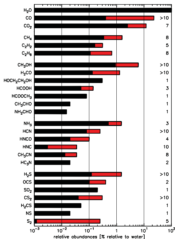
Figure 1. Abundances relative to water of cometary parent molecules. The range of measured values is shown in the gray (red in the color version) portion. The number of comets in which the molecule has been detected is given in the right (adapted from Bockelée-Morvan et al. (2005), courtesy J. Crovisier).
