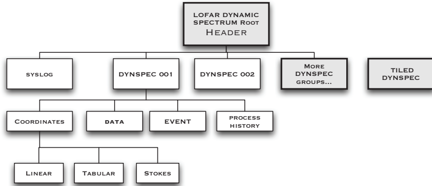
Figure 2. LOFAR Dynamic Spectra Data Structure.
