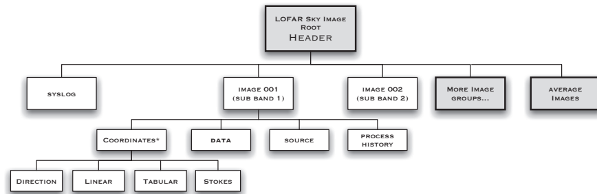
Figure 1. LOFAR Radio Sky Image Data Structure.
