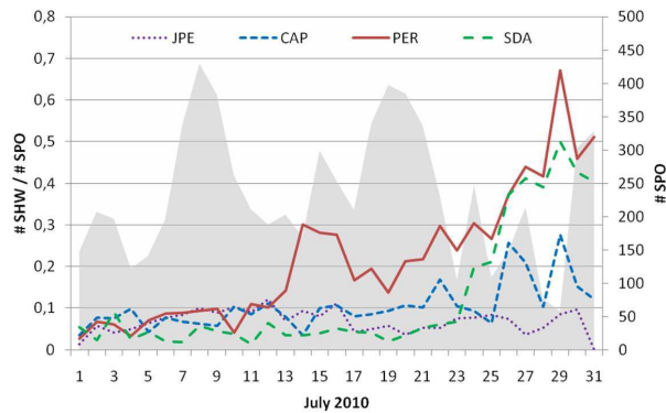
Figure 2 – Activity profile of the July Pegasids, \alpha -Capricornids, Perseids, and Southern \delta -Aquariids in July 2010. Plotted is the number shower meteors per night, divided by the number of sporadics. The absolute number of sporadic meteors is given in the background.
