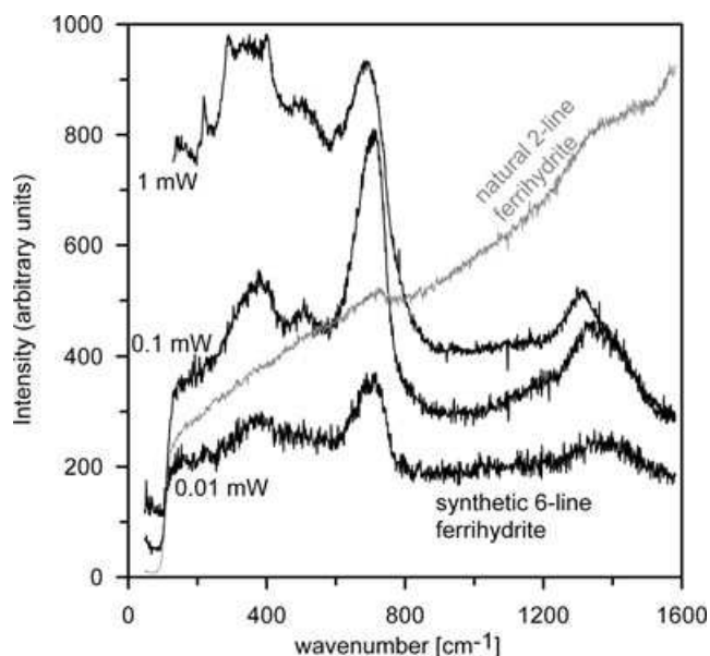
Figure 5. Three Raman spectra of six-line ferrihydrite, measured at different laser powers: 0.01 mW, 30 min; 0.1 mW, 15 min; 1 mW, 10 min. At the lowest power, the 510 \text{cm}^{-1} band is not discernible. At 1 mW, the spectrum starts to change because the mineral is transformed. The two-line sample contains organic matter, which leads to fluorescence. Only the band at 710 \text{cm}^{-1} is discernible (0.1 mW, 10 min). A similar, albeit weaker, spectrum can be produced at 0.01 mW with an integration time of 30 min.
