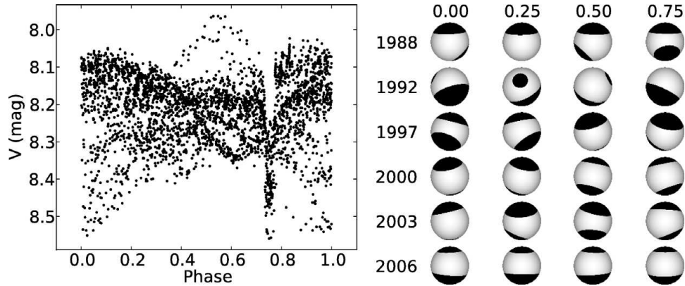
Figure 1. Almost all of the photometric variability of a magnetically active star is related to starspots. The light curve (left panel) of the spotted binary star HD 6286 shows 20 years of V-band data from the 0.75m Vienna-T7 and the 0.40m Tennessee-T3 Automatic Photoelectric Telescope, both located in southern Arizona. All data were phased with the rotation period of the primary component and demonstrate the continuous and systematic variability of the star as shown in the spot-model solutions to the right. Note that HD 6286 is an eclipsing binary with primary minimum at phase 0.75.
