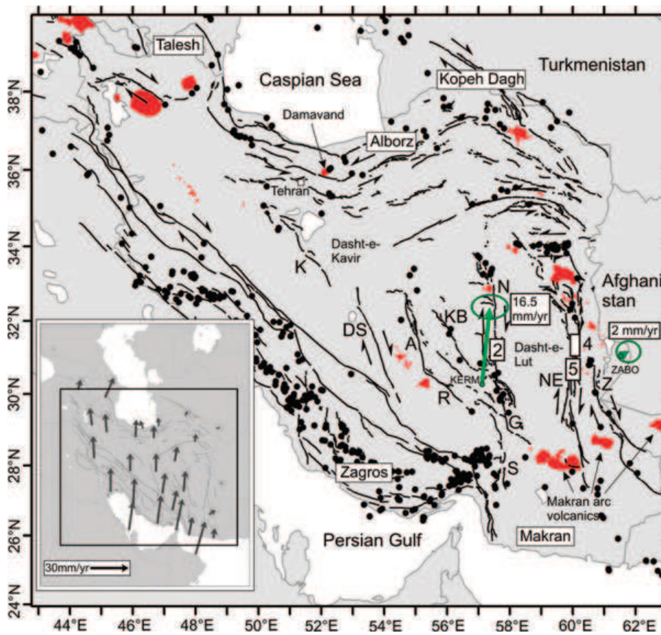
Figure 1. Map of Iran showing the distribution of active faults, earthquake epicentres (magnitude >5, from the catalogue of Engdahl et al. 1998 and its subsequent updates) and outcrops of Plio-Quaternary volcanic rocks (from Emami et al. 1993). Plio-Quaternary volcanism (marked in red) is widespread across eastern and central parts of the country. An east–west alignment in active volcanoes north of the Makran mountains represents volcanism from active subduction of oceanic lithosphere of the Arabian sea. Volcanic centres within the interior of Iran appear to show either an NW–SE alignment or appear to be closely associated with zones of presently active faulting (for instance, around the Dasht-e Lut desert). GPS velocities of points relative to Eurasia, shown in the inset, are from Vernant et al. (2004). The GPS velocities (relative to Eurasia) of stations KERM and ZABO, which together define the 16 \pm 2 \text{ mm yr}^{-1} rate of north–south right-lateral shear across eastern Iran, are included on the main map for clarity (in green). Active faults are labelled as follows: Z = Zahedan; NE = Neh faults (East and West Neh); S = Sabzevaran; G = Gowk; N = Nayband; KB = Kuh Banan; R = Rafsanjan; A = Anar; DS = Deh Shir; K = Kashan. The Neh and Zahedan faults east of the Dasht-e Lut desert are situated within the Sistan Suture Zone.
