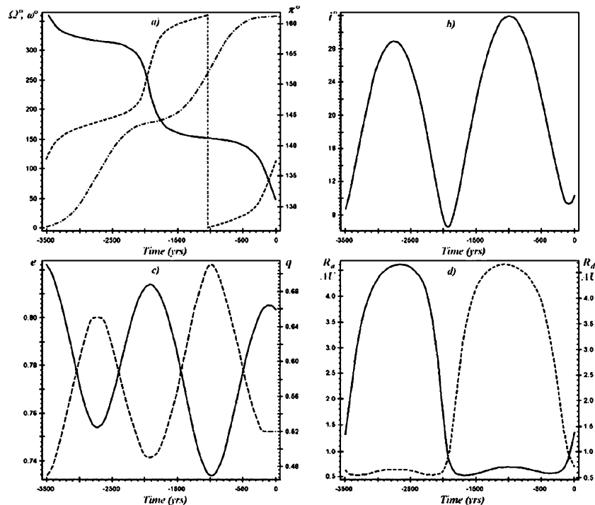
Figure 1. The variation with time in the orbital elements of NEO 1998VD31. Plot (a) shows the variation of three angular elements \omega (—), \Omega (---), \pi (· · ·). Plot (b) shows the variation of the inclination i . Plot (c) shows the variations of the eccentricity e and the perihelion distance q (---). Plot (d) shows the variation of the two heliocentric nodal distances, R_a -ascending node and R_d -descending node (---).
