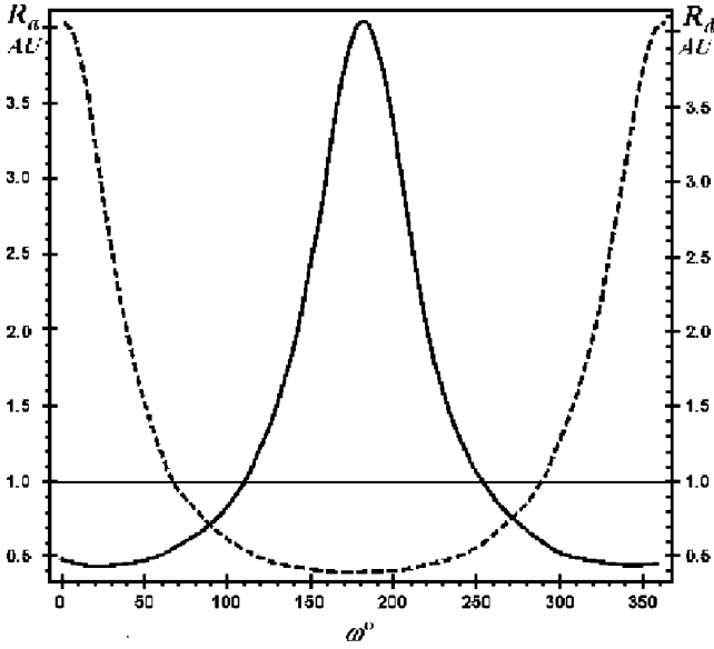
Figure 2. The variation in heliocentric distance of the ascending node R_a and descending node R_d (---) plotted against the argument of perihelion \omega for NEO 2003UL3.
