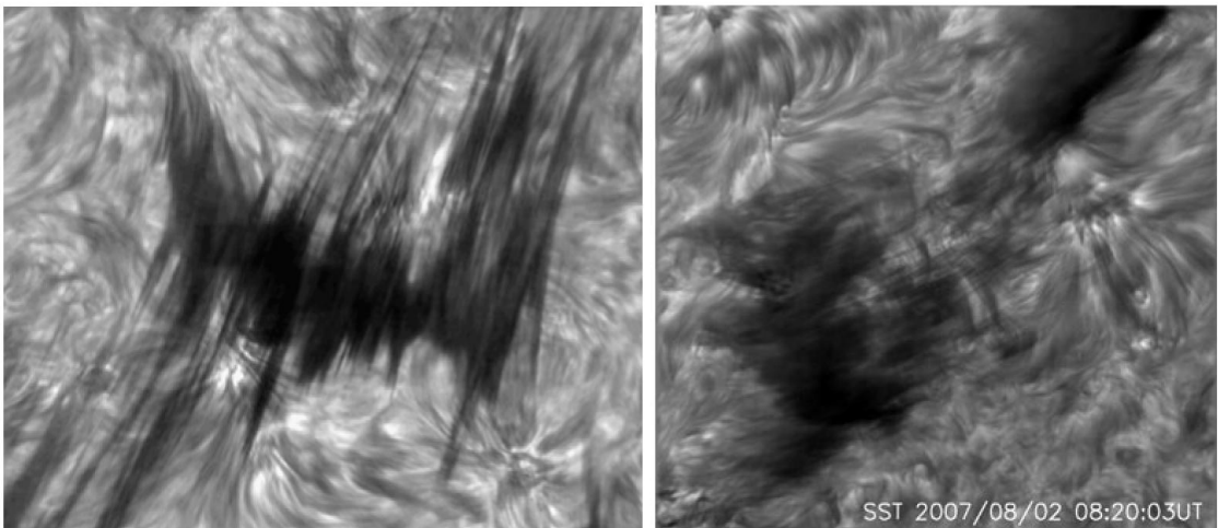
Figure 1. High resolution H\alpha filtergrams of two quiescent solar filaments obtained with the Swedish Solar Telescope at La Palma. Left: Close to disk center August 22, 2004. Right: SW quadrant August 2, 2007.
