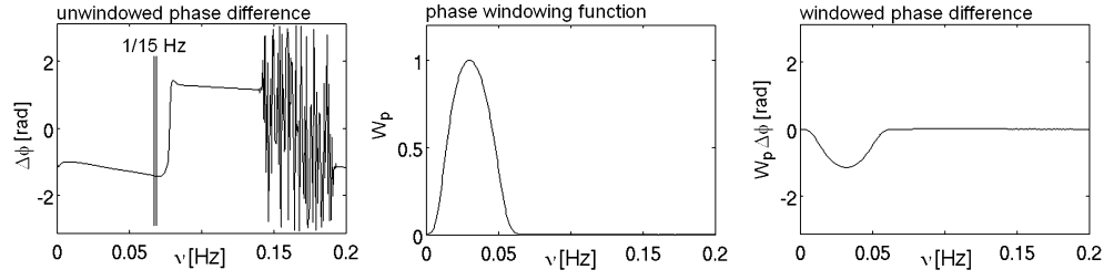
Figure 2. Left-hand panel: unweighted phase difference \Delta\phi at t = 450 s. Central panel: phase weighting function W_p = \log(1 + |\tilde{u}^0|)/\max \log(1 + |\tilde{u}^0|) at t = 450 s. Right-hand panel: windowed phase difference W_p\Delta\phi at t = 450 s.
