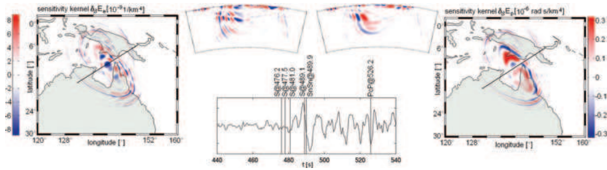
Figure 10. The same as Fig. 10 but for the S-wave train.
