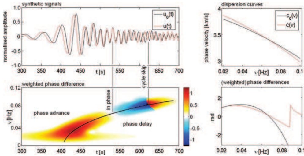
Figure 1. Upper left-hand panel: time-domain signals u^0(t) plotted in black and u(t) plotted in red. Upper right-hand panel: dispersion curves c(\nu) and c^0(\nu) in the frequency range that contributes to u(t) and u^0(t) (see eqs 13). Lower left-hand panel: weighted phase difference W_p \Delta\phi as a function of time t and frequency \nu . The weighting function is W_p = \log(1 + |\tilde{u}^0|) / \max \log(1 + |\tilde{u}^0|) . Vertical lines indicate the times when the signals are in phase and phase shifted by -\pi , respectively. The bold line traces the extremal weighted phase differences for a given frequency. Those values are plotted separately in the lower right-hand panel (red line). The weighted phase difference is compared with the phase difference -\omega x/c(\omega) + \omega x/c^0(\omega) plotted in black.
