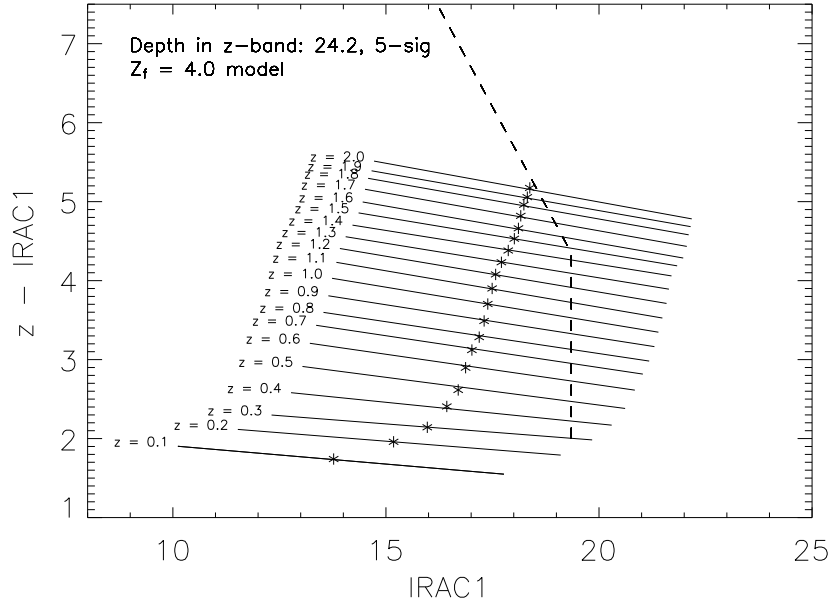
Figure 2. Simulated red-sequences for a z' -[3.6] filter combination assuming a Bruzual & Charlot (2003) model where a galaxy undergoes a burst of star-formation at z_f = 4.0 and evolves passively thereafter. The dashed line is the depth of our survey. M_* the characteristic magnitude at each redshift is denoted by an asterisk. Photometric redshifts can be determined from the red-sequence ( z' - [3.6] ) color) to an accuracy of 10%.
