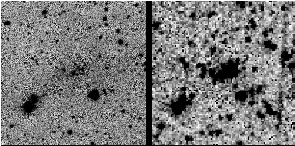
Figure 3. z' (left) and [3.6] (right) image of a z = 1.22 cluster in the 6 \text{ deg}^2 “pilot patch” (the redshift is estimated from the color). The FOV is 1 Mpc at the cluster center. For a color image and more examples see ( http://spider.ipac.caltech.edu/staff/gillian/SpARCS ). Note: This cluster was discovered independently by the XMM-Newton Large Scale Structure Survey (Pierre et al. 2004).
