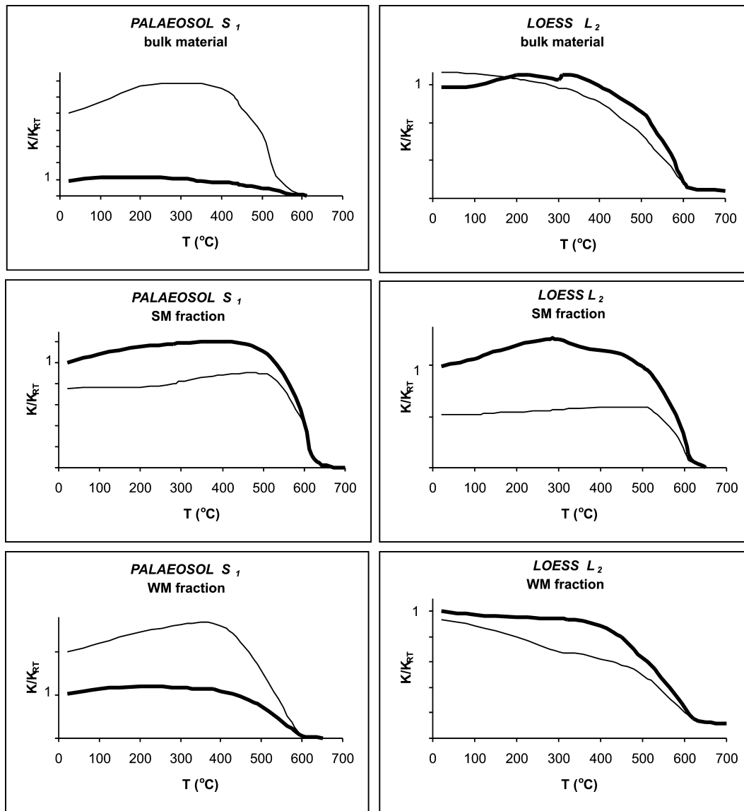
Figure 6. Thermomagnetic analyses of magnetic susceptibility K(T) for the S_1/L_2 couplet: (a) bulk material of S_1 , (b) bulk material of L_2 , (c) strongly magnetic (SM) fraction of S_1 , (d) strongly magnetic (SM) fraction of L_2 , (e) weakly magnetic (WM) fraction of S_1 and (f) weakly magnetic (WM) fraction of L_2 . Susceptibility is normalized to the initial value at room temperature (RT). Heating curves denoted by solid circles, cooling curves by thin lines.
