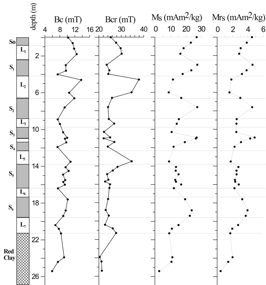
Figure 8. Variations of the coercivity parameters B_c and B_{cr} , saturation magnetization ( M_s ) and saturation remanence ( M_{rs} ) with depth in the Viatovo section.
