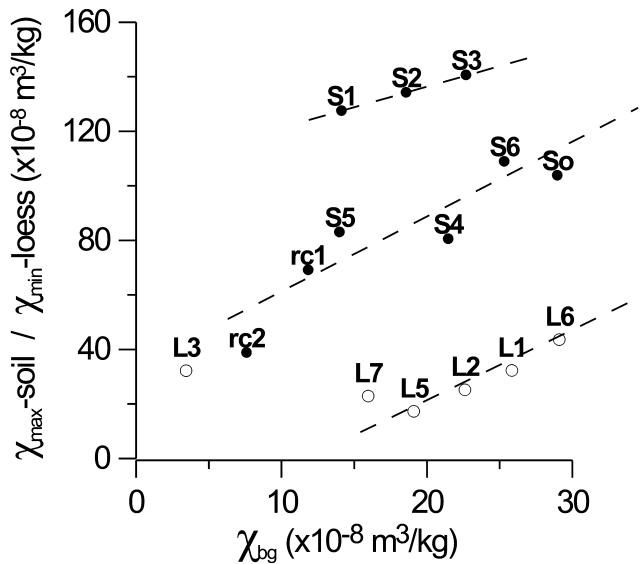
Figure 3. Relationship between the calculated background magnetic susceptibilities ( \chi_{bg} ) in different loess and soil units of the Viatovo section and the corresponding minimum (for loesses) and maximum (for palaeosols) susceptibility values found within the separate units. The abbreviations rc1 and rc2 refer to the two red clay units, which can be discriminated by their susceptibilities (see Fig. 2).
