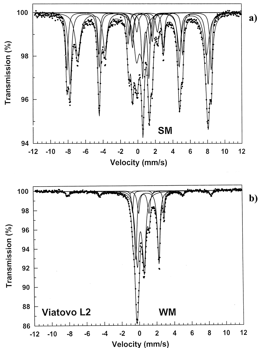
Figure 7. Room temperature (RT) Mössbauer spectra of a sample from loess unit L 2 (a) SM fraction and (b) WM fraction.
