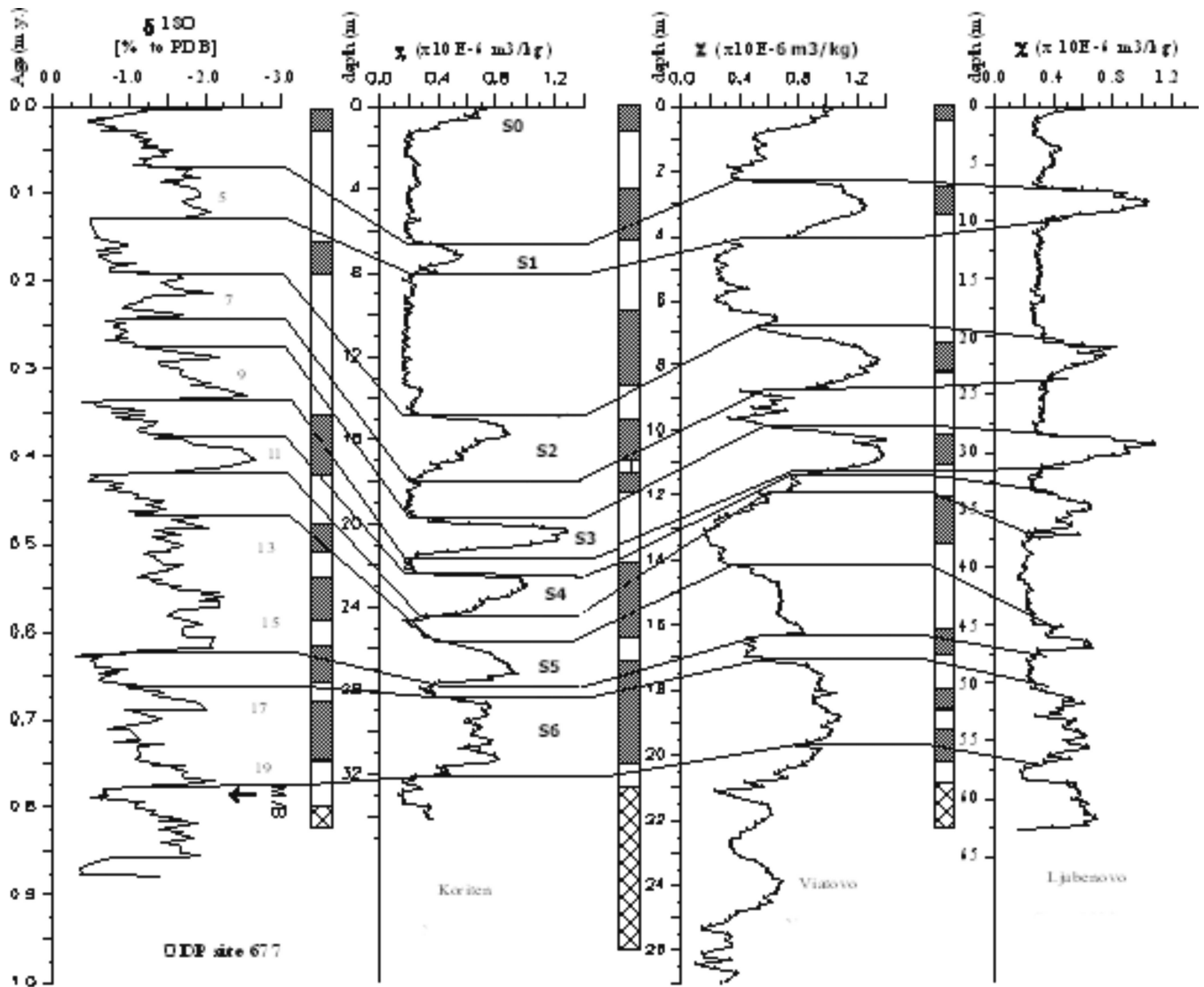
Figure 9. Correlation of the magnetic susceptibility of three loess/palaeosol sequences in Lubenovo (unpublished results), Viatovo and Koriten in Northern Bulgaria (see Fig. 1 for the locations) with the astronomically tuned \delta^{18}\text{O} record from ODP site 677 of Shackleton and Hall (1989).
