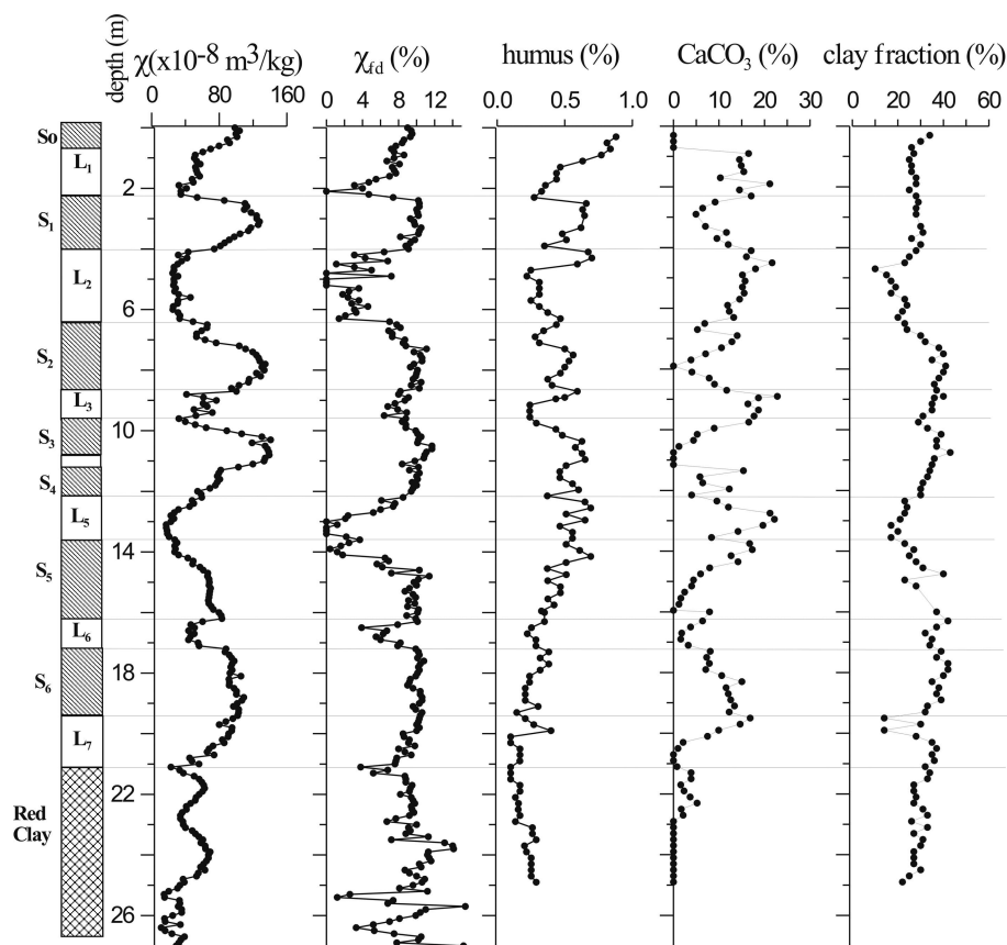
Figure 2. Depth variations of low-field magnetic susceptibility, percent frequency dependent susceptibility, humus, calcium carbonate ( \text{CaCO}_3 ) and clay content at Viatovo.
