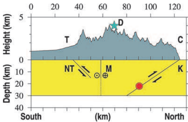
Figure 10. A section across the Alborz from near Tehran (T) at 35.5^{\circ}\text{N} 51.3^{\circ}\text{E} to near Chalus (C) at 36.8^{\circ}\text{N} 51.8^{\circ}\text{E} . The top is the vertically-exaggerated topography, shaded in gray. The blue star marked D is the projected position of Damavand volcano on this line of section. Beneath the topography, with equal vertical and horizontal scales, are shown the downward projections of the Khazar (K), Mosha (M) and North Tehran (NT) faults. The red circle is the approximate mainshock hypocentre (HDC epicentre plus 22 km centroid depth) for the 2004 Baladeh earthquake projected on to the line of section. The yellow layer is to illustrate a seismogenic layer 30 km thick: it does not represent the crustal thickness, which is about 40–50 km in the central Alborz. The aim is to show that even if the seismogenic layer was as thick as 30 km, the Khazar and Mosha faults are unlikely to intersect within the seismogenic layer. The North Tehran and Mosha faults may intersect within the seismogenic layer, depending on its thickness on the southern side of the Alborz and on the dip of the North Tehran Fault: see text for discussion.
