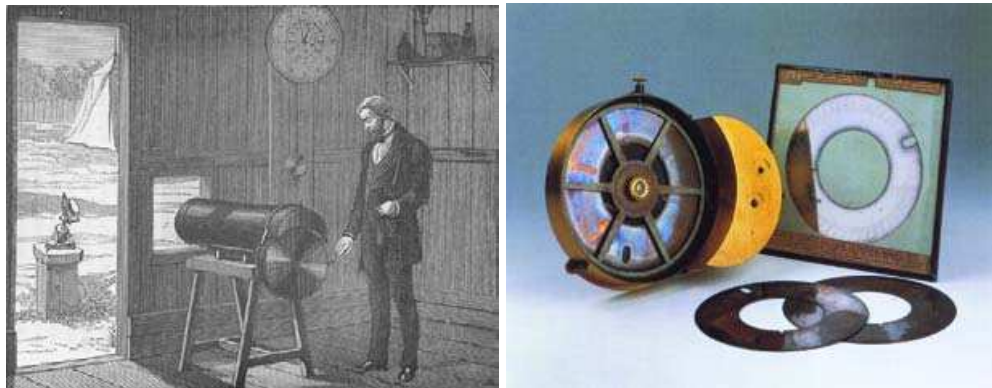
Figure 1. (Left panel) Francisco Antônio de Almeida. The Brazilian astronomer was commissioned and sent by Conde Prados, director of the Imperial Observatory of Rio de Janeiro, to study astronomy in France, when he was invited to participate in the French commission in Nagasaki, where he was responsible for the use of Jules Janssen’s photographic revolver (1824–1907). With this device it was possible to obtain very close pictures that were produced on a type of film through which Venus was visualized in front of the Sun. (Right panel) Photographic revolver built by R dier, used in Nagasaki in 1874. This invention is considered one of the prototype of the today’s movies.
