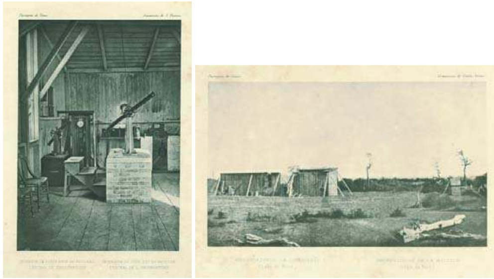
Figure 3. (Left panel) The Commission of St Thomas, West Indies: interior of the east part of the central pavilion of the Brazilian Observatory. In this place the passage of the planets was observed by the meridian. From that observation rigorous determination of the local time was made, a fundamental factor to accurately measure the contact of Venus entering the disk of the Sun. (Right panel) The Commission of Punta Arenas, Chile: The Brazilian astronomer of Belgian origin Luiz Cruls was the chief of the Brazilian mission to Punta Arenas. The clear visibility of the Chilean sky allowed the whole phenomenon to be registered.
