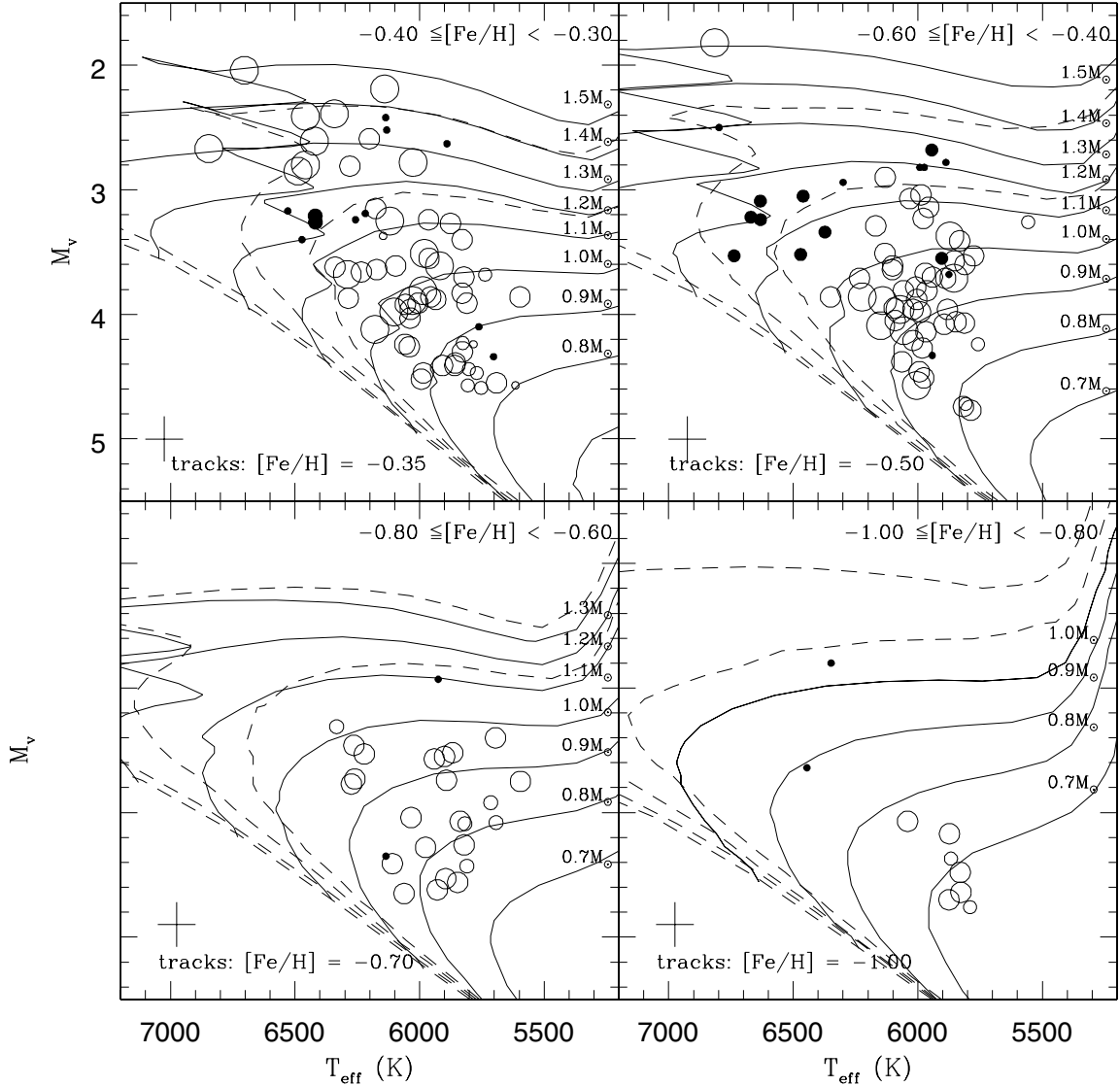
Figure 2. H–R diagrams showing stars from Table 1 for the four bottom [\text{Fe}/\text{H}] bins. See caption to Fig. 1 for further explanation.
