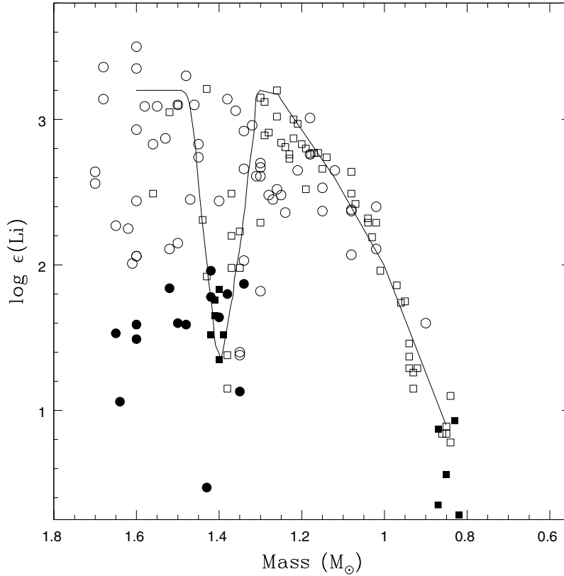
Figure 4. Lithium abundance versus stellar mass for the Hyades members (open squares) and field stars with [\text{Fe}/\text{H}] in the range 0.0 to +0.2 (circles). Filled symbols denote upper limits to the lithium abundance. The solid line is the mean relation for the Hyades stars with the Li dip prominent at about M = 1.4 M_{\odot} .
