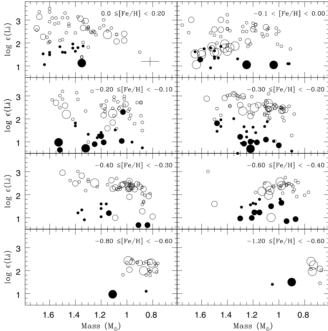
Figure 3. Li abundance versus stellar mass in eight different [\text{Fe}/\text{H}] bins. Filled circles denote upper limits to the lithium abundance. Open circles refer to measured abundances. The three sizes for the circles identify the accuracy of the Hipparcos parallax, a major influence on the derived mass. Stars with a parallax error \geq 10 per cent are assigned the biggest circle. Stars with an error of 5 to 10 per cent are shown with the middle-sized circle. Those stars with a 5 per cent or smaller error are given the smallest circles.
