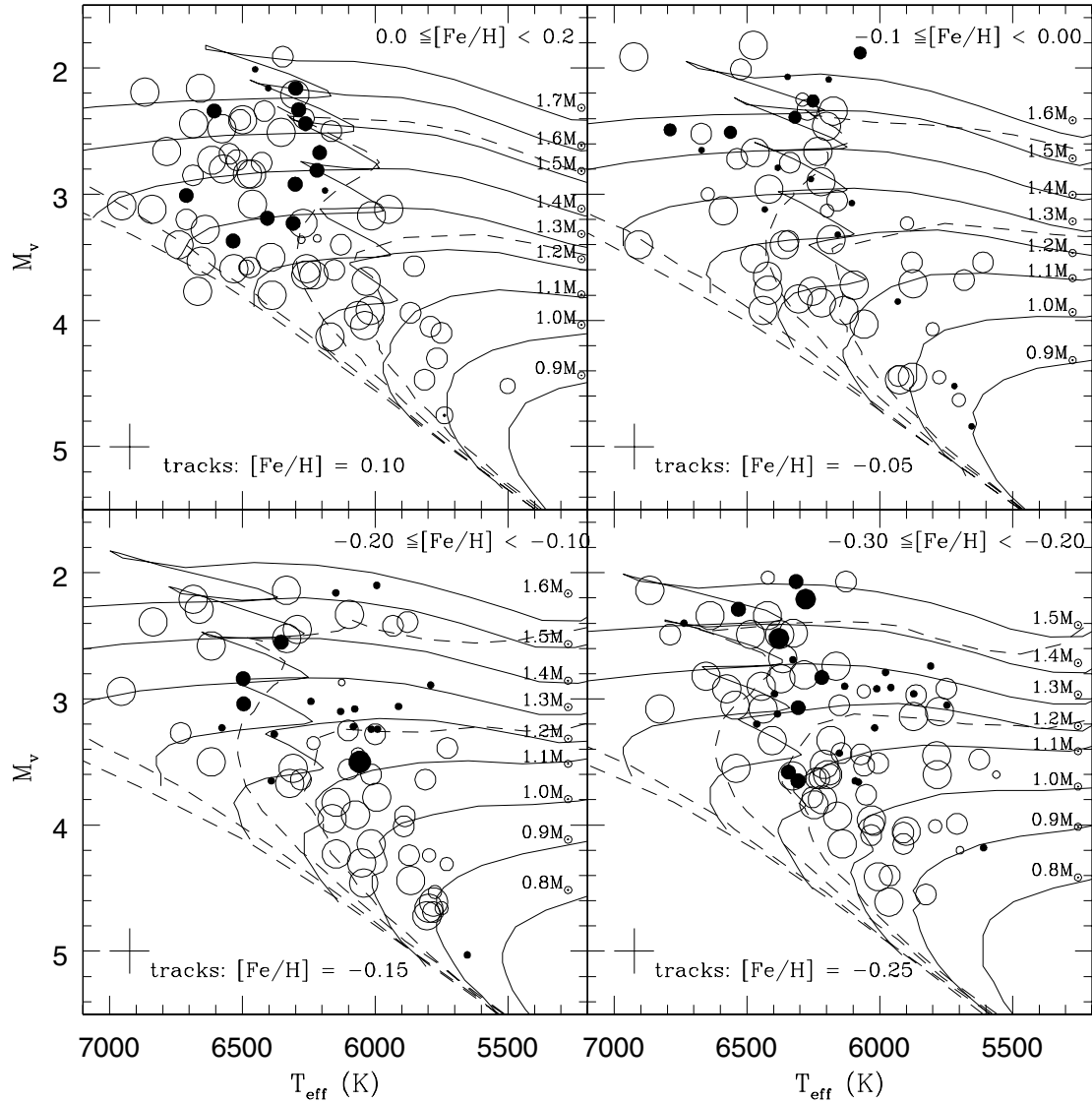
Figure 1. H–R diagrams showing the stars from Table 1 for the top four metallicity bins. Evolutionary tracks (solid lines), and isochrones (broken lines) for 100, 700, 2500, and 4500 Myr from Girardi et al. (2000) are shown for the mean [\text{Fe}/\text{H}] of a bin. Filled circles denote stars with no detected lithium, and open circles denote stars with detectable lithium. The symbol size represents the magnitude of the lithium abundance (or upper limit). Four sizes are used. In order of decreasing symbol size, the abundance intervals are: \log \epsilon(\text{Li}) \geq 2.50 , 2.0 \leq \log \epsilon(\text{Li}) < 2.5 , 1.5 \leq \log \epsilon(\text{Li}) < 2.0 , and \log \epsilon(\text{Li}) < 1.5 .
