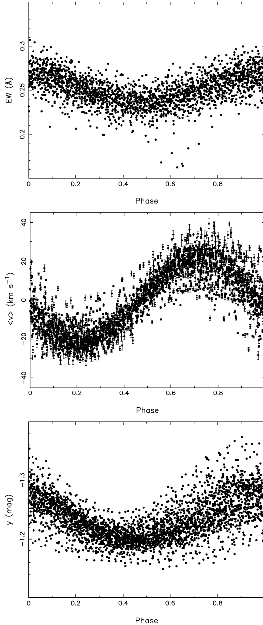
Figure 4. Phase diagram according to f_1 of the equivalent width of the Si III \lambda 4553 Å line (top), of the radial velocity (including standard errors derived from averaging over the three Si lines of the triplet, middle) and of the Strömgren y data taken from Paper I (bottom). The reference epoch was each time taken to be HJD 245 2500.
