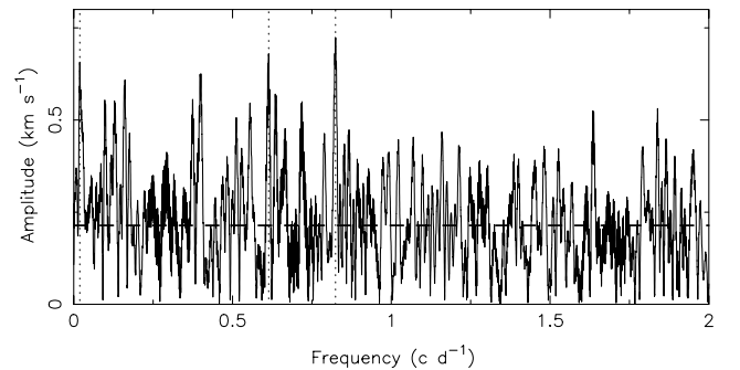
Figure 6. Amplitude spectrum of \nu Eridani computed from residual radial velocities after pre-whitening with the 19 frequencies listed in Table 2. The dotted lines indicate the frequencies f_{19} , f_{20} and f_{21} given in Table 3. The dashed horizontal line indicates the noise level as defined in the text. We refer to the text for further details.
