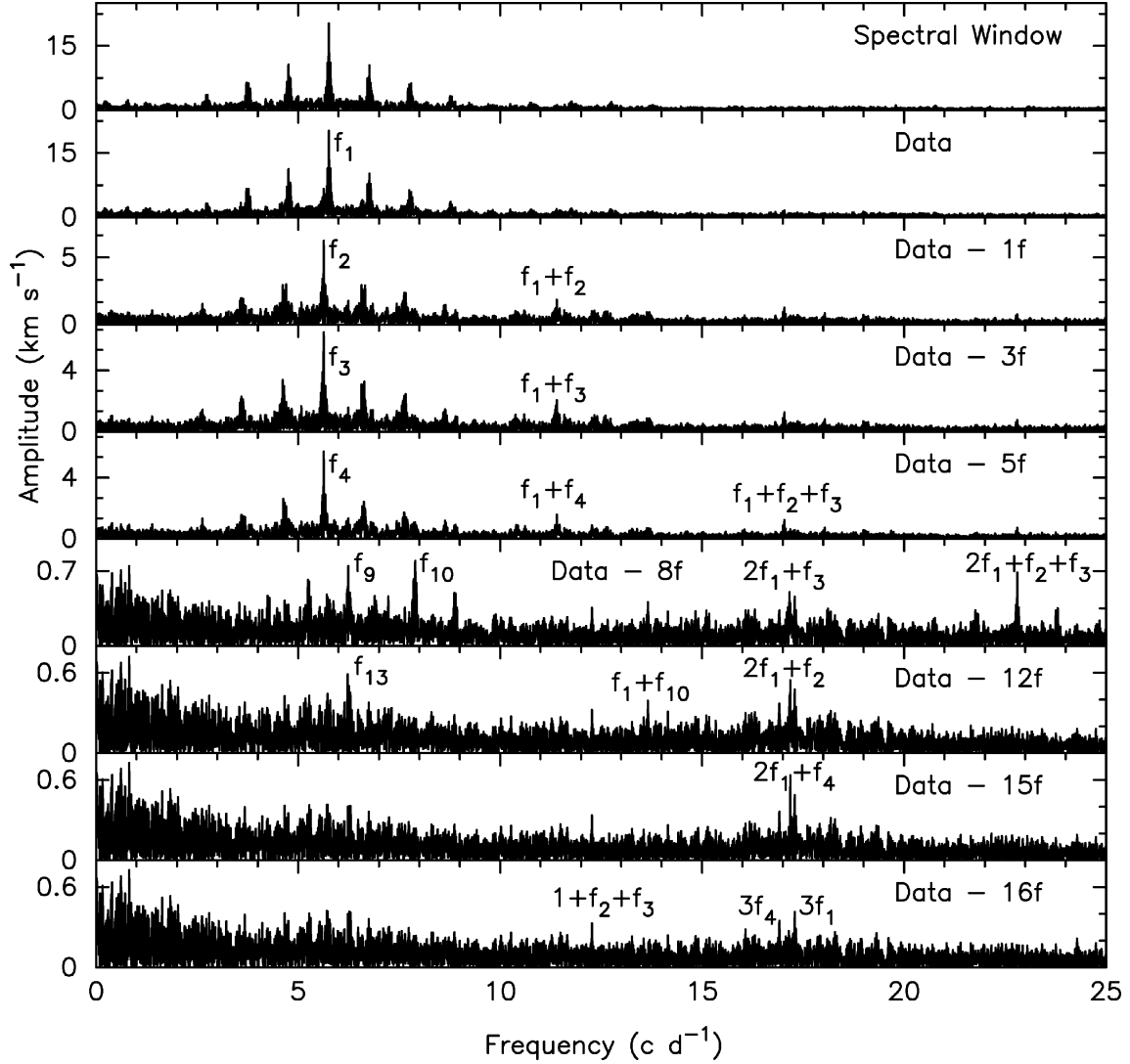
Figure 5. Amplitude spectra of \nu Eridani computed from the radial velocities. The uppermost panel shows the spectral window of the data. All subsequent panels show the periodograms after different stages of pre-whitening (note the different scale). We refer to the text for details.
