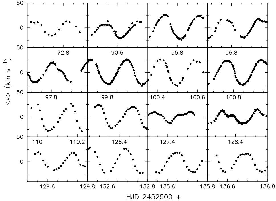
Figure 3. Radial velocities of \nu Eridani during some selected nights of the dedicated multisite campaign.
