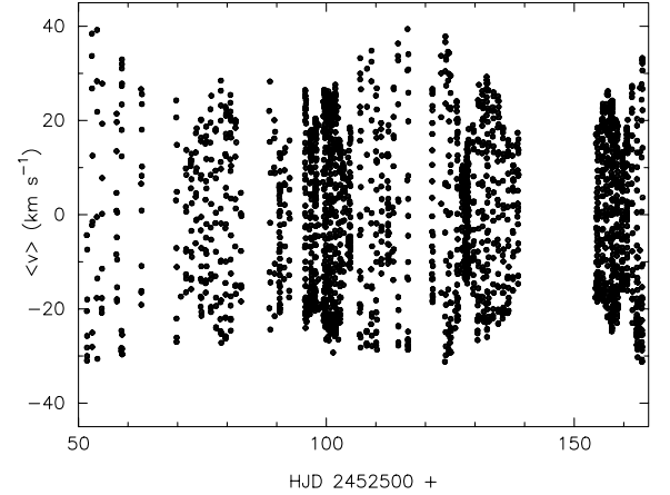
Figure 2. The time series of the average Si III radial velocities of \nu Eridani derived from each spectrum taken during the dedicated multisite campaign.
