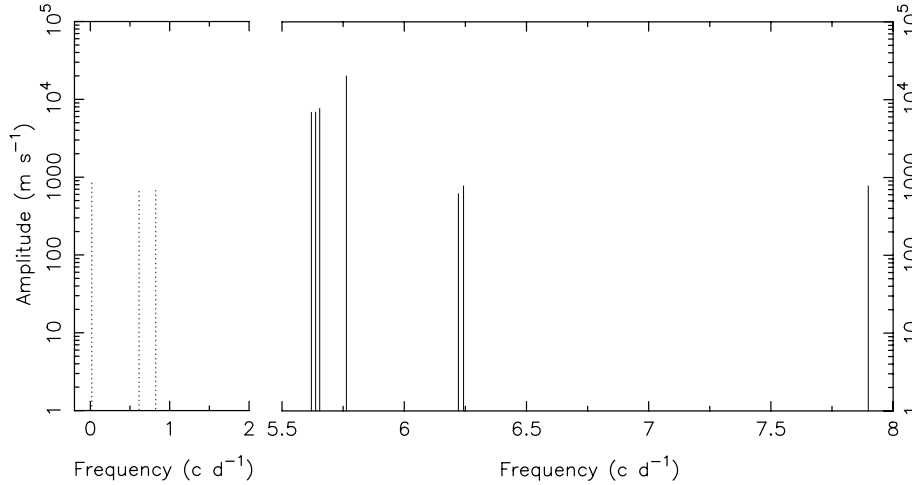
Figure 7. Final amplitude spectrum of the intrinsic frequencies derived from the radial velocities. The unambiguous intrinsic frequencies listed in Table 2 are indicated by a full line while the uncertain frequencies given in Table 3 are represented by the dotted lines. We stress that the x -axis is interrupted and has a different scale for both panels. Moreover, the y -axis is logarithmic and we have expressed the amplitudes in \text{m s}^{-1} in order to suppress the dominance of the main mode in the graph.
