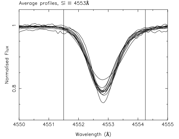
Figure 1. The average profile of the Si III \lambda 4553 Å line of \nu Eridani plotted for each of the observatories separately.
