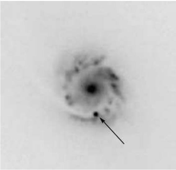
Figure 4. The annulus of H II regions and hotspots surrounding the nucleus of NGC 1097, possibly a region of intense star formation. The frame was taken on 1992 October 16 with NTT + EMMI (filter R) and includes the Type II SN 1992bd, indicated by an arrow. NGC 1097 also hosted SN 1999eu, studied in this paper, as well as the Type II SN 2003B.
