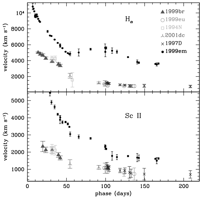
Figure 20. Photospheric velocity of low-luminosity Type II SNe deduced from the minima of P-Cygni absorption of H\alpha and Sc\ II\ 6246\ \text{\AA} and comparison with SN 1999em (data from the Padova-Asiago SNe Archive and Leonard et al. 2002a). The x-axis shows the phase with respect to explosion.
