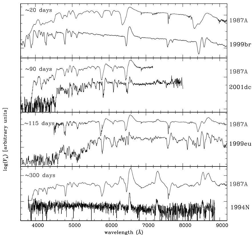
Figure 21. Comparison of the spectra of SN 1987A with those of faint Type II SNe at similar phases. The phases with respect to the explosion epoch are shown in the upper-left corner.
