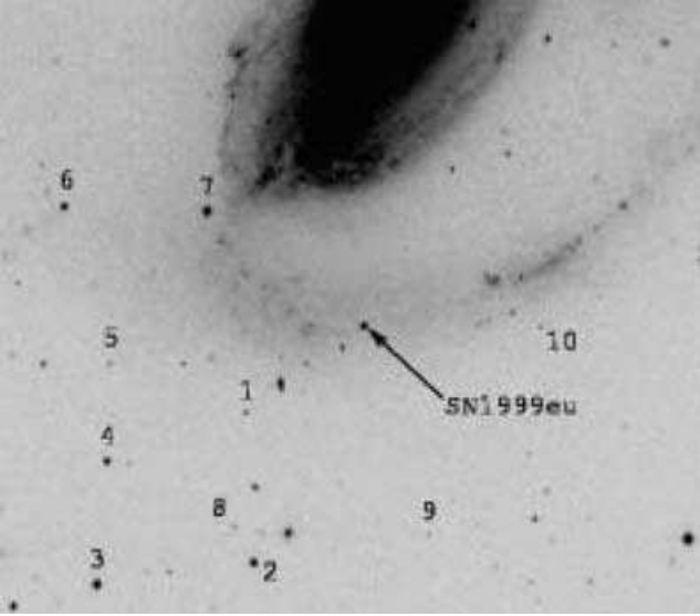
Figure 3. SN 1999eu in NGC 1097 ( R -band image with ESO-Danish 1.54-m telescope + DFOSC).
