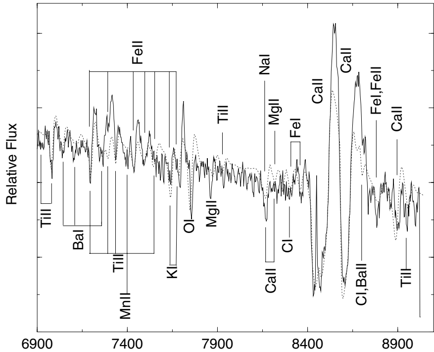
Figure 26. Like Fig. 24, but in the wavelength range \lambda\lambda 6900\text{--}9000 .
