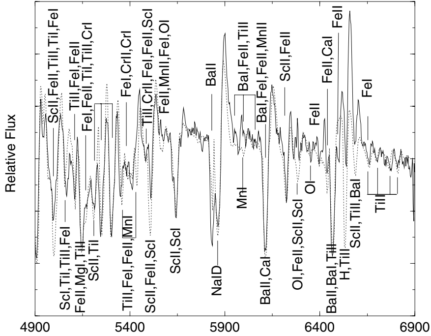
Figure 25. Like Fig. 24, but in the wavelength range \lambda\lambda 4900\text{--}6900 .
