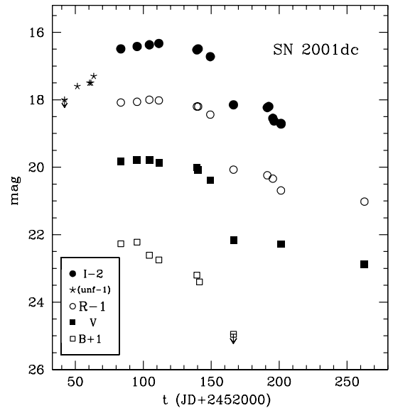
Figure 9. BVRI light curves of SN 2001dc. The unfiltered precovery limit and magnitudes (asterisks) are shown with respect to the R -magnitude scale (Hurst et al. 2001). The magnitude at phases later than ~100 d are affected by large errors.
