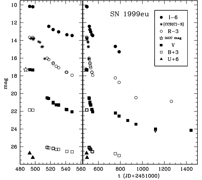
Figure 5. BVRI light curves of SN 1999eu. Left: enlargement of the first two months. Right: complete light curves. Two points in the U band are also reported. The star (plotted with respect to the V magnitude scale) refers to the discovery unfiltered magnitude (IAUC 7304 Nakano & Aoki 1999). The asterisks are taken from the web sites http://aude.geoman.net/observation/SN/infc99eu.htm and VSNET ( http://www.kusastro.kyoto-u.ac.jp/vsnet/ ), and are plotted with respect to the R -magnitude scale.
