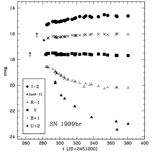
Figure 2. UBVRI light curves of SN 1999br showing its extended plateau. Two predisccovery limits (IAU Circ. 7143), unfiltered measurements, are also shown placed to correspond with the R -magnitude scale (IAU Circ. 7141). Photometry from Hamuy et al. (in preparation) is also shown.
