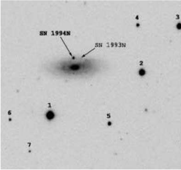
Figure 6. SN 1994N and the Type IIin SN 1993N in UGC 5695 ( R -band image taken with the ESO 3.6-m telescope + EFOSC1 on 1994 May 9).
