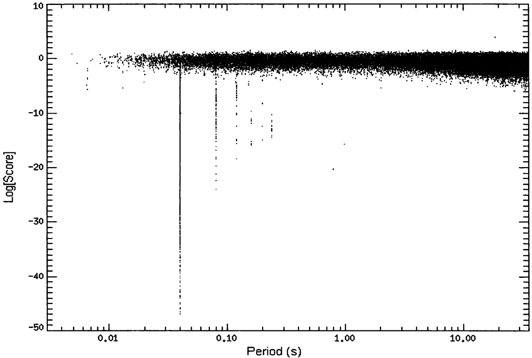
Figure 2. Score distribution vs. period for pulse candidates.
