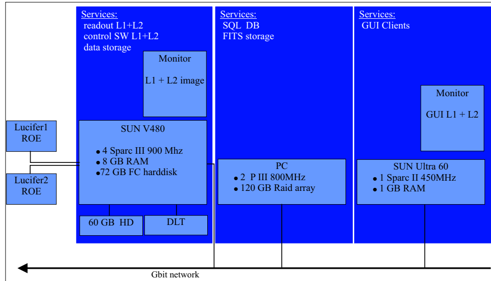
Figure 2. Hardware architecture and services.
