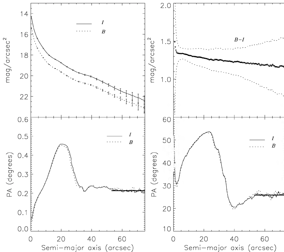
Figure 5. As in Fig. 2 but for NGC 1440.
