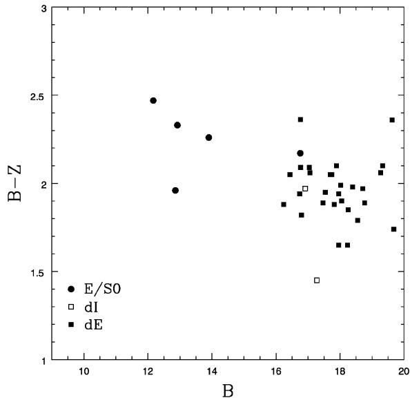
Figure 8. Colour–magnitude diagram for the 35 galaxies that were in the nine fields observed in Z and bright enough to be detected at the 5\sigma level in the Z data. All magnitudes were measured in an aperture of radius 6 arcsec, which was large enough that the effect on the colours caused by differential seeing between the B and Z data was negligible. Only galaxies with total absolute magnitudes of M_B < -12 are shown. Fainter (and consequently lower surface brightness galaxies) were not detected above sky in the Z-band data, particularly since that data suffers from serious fringing, typically 6 per cent of the sky ( http://www.ast.cam.ac.uk/~wfcsur/defringing.html ). Dwarf elliptical galaxies have B - Z colours of 1.7–2.2 given the spectral energy distributions of Trentham et al. (1998b).
