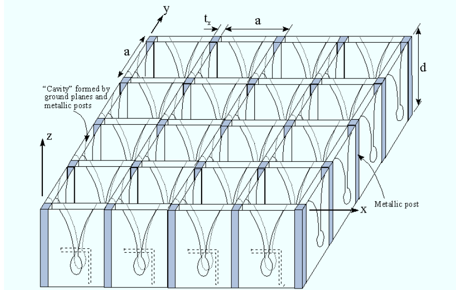
Figure 5. Dual-polarized array with conducting posts at corners of unit cells.
