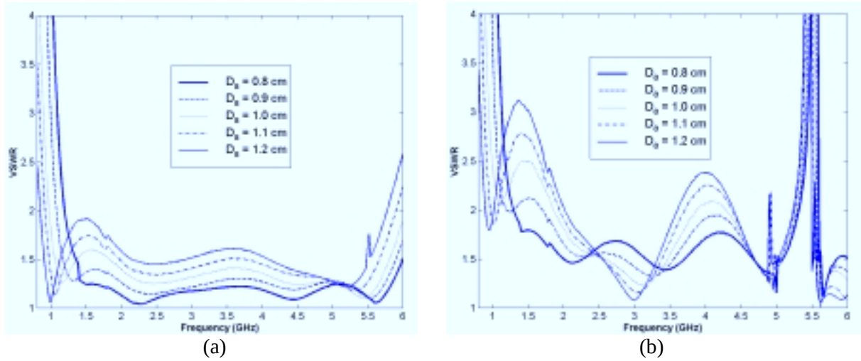
Figure 7. Effects of slotline cavity for array scanned to (a) 45° in E-plane and (b) 45° in H-plane. Antenna parameters as in Figure 6.
