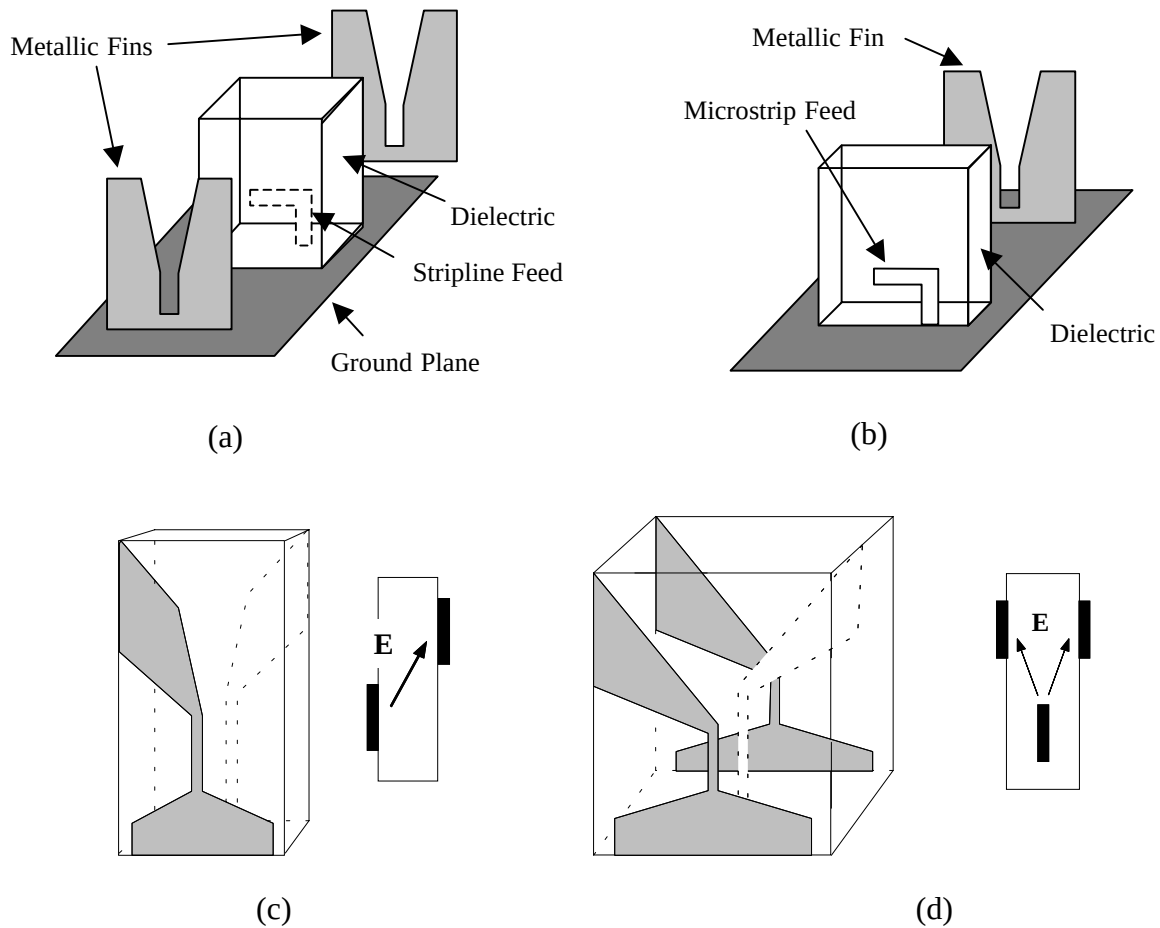
Figure 1. Some variations of the original tapered slot antenna configuration. (a) stripline version consisting of two ground planes and one stripline feed, (b) microstrip versions consisting of one substrate with a ground plane on one side and a microstrip conductor on the other, (c) antipodal antennas consisting of a gradual transition from microstripline to antipodal strips and then to antipodal flared radiators, and (d) balanced antipodal antennas that utilize stripline feed and a second ground plane with tapered metalization.
