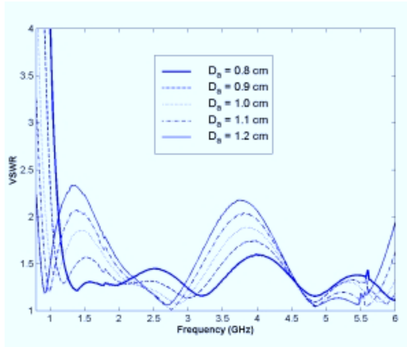
Figure 6. SWR for dual-polarized arrays with various slotline cavity diameters. Beam pointed to broadside. Element configuration as in Fig. 4; L_s = 4.5 cm, w = 2.0 cm, R = 0.3 cm -1 .
