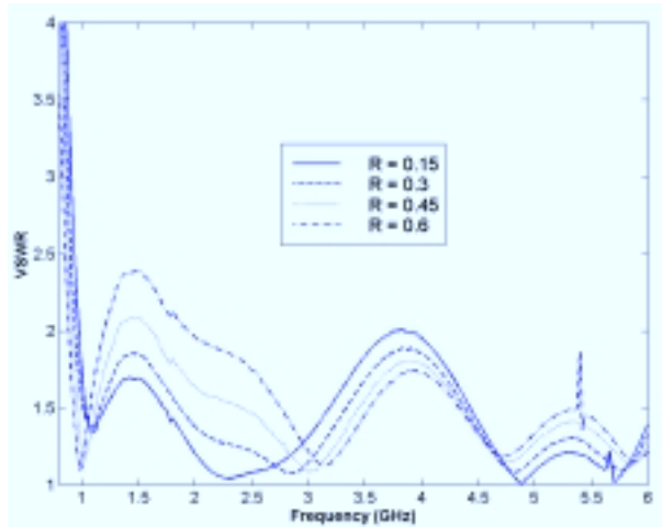
Figure 8. Effects of exponential opening rate. Antenna parameters same as Fig. 6; D_a = 1.0 cm.
