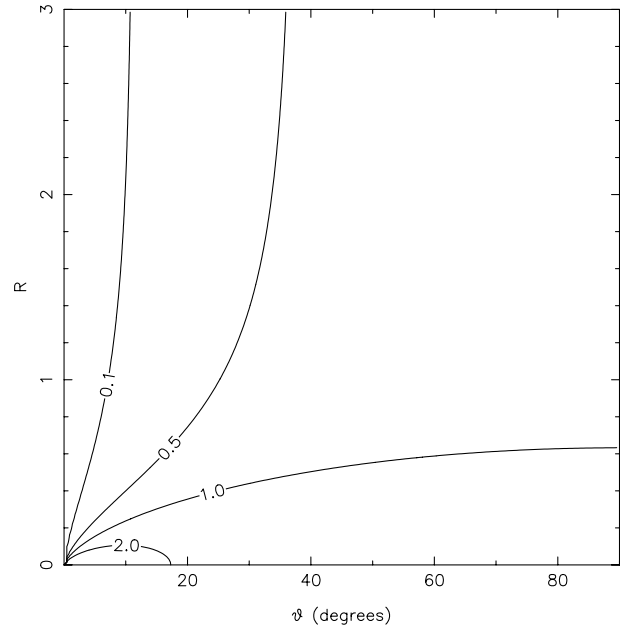
Figure 3. Contours of \mathcal{K} , the ratio between projection-corrected and inferred ratios of thermal to radio pressure, as a function of R and \theta . The figure is calculated for \beta = 0.67 ; similar results are obtained with \beta = 0.5 and 0.9 .
