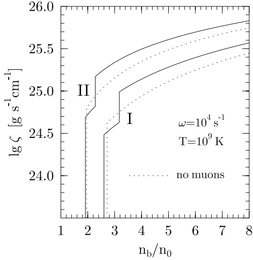
Fig. 2. The bulk viscosity \zeta_0 for models I and II of non-superfluid npe\mu matter (solid lines) induced by the non-equilibrium direct Urca processes involving electrons and muons versus the baryon number density n_b , for T = 10^9 K and \omega = 10^4 s ^{-1} . Dotted lines show the same bulk viscosity but for the simplified models of matter without muons.
