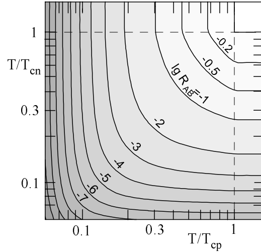
Fig. 5. Same as in Fig. 4 but for the case in which the superfluidity of nucleons 1 is of type A while the superfluidity of nucleons 2 is of type B.
