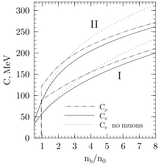
Fig. 1. Linear response of chemical potential difference to baryon number density perturbation, C_l = n_b \partial \eta_l / \partial n_b , versus the baryon number density n_b for two model equations of state proposed by Prakash et al. (1988) and discussed in the text. Solid curves correspond to l = e , while dot-and-dash curves to l = \mu . Dotted lines present C_e for the simplified models of matter without muons.
