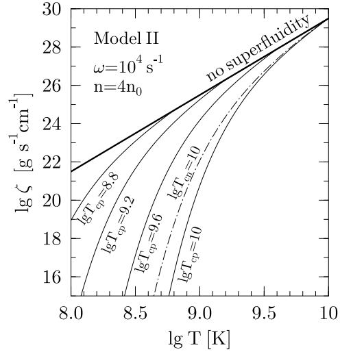
Fig. 7. Bulk viscosity \zeta of superfluid npe\mu matter (model II) produced by the electron and muon direct Urca processes at the baryon number density n_b = 4n_0 and \omega = 10^4 \text{ s}^{-1} as a function of temperature for non-superfluid matter (thick solid line), for matter with superfluid protons (solid curves, T_{cp} = 10^{10} , 10^{9.6} , 10^{9.2} and 10^{8.8} ) and normal neutrons, and for matter with superfluid neutrons (dash-and-dotted curve, T_{cn} = 10^{10} \text{ K} ) and normal protons.
