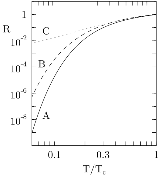
Fig. 3. Reduction factors R of the bulk viscosity versus \tau = T/T_c for three superfluidity types A, B and C (Table 1).
