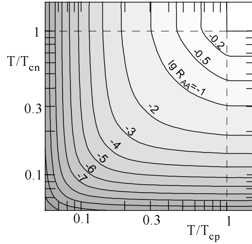
Fig. 4. Isolevels of the reduction factor R of the bulk viscosity by nucleon superfluidity of type AA versus \tau_1 = T/T_{c1} and \tau_2 = T/T_{c2} . In the domain \tau_1 \geq 1 , \tau_2 \geq 1 nucleons 1 and 2 are normal and R_{AA} = 1 . In the domain \tau_1 < 1 , \tau_2 \geq 1 nucleons 1 are superfluid and nucleons 2 normal, while in the domain \tau_1 \geq 1 , \tau_2 < 1 nucleons 1 are normal and 2 superfluid; in these domains R depends on one parameter ( \tau_1 or \tau_2 ). In the domain \tau_1 < 1 , \tau_2 < 1 both nucleons 1 and 2 are superfluid at once.
