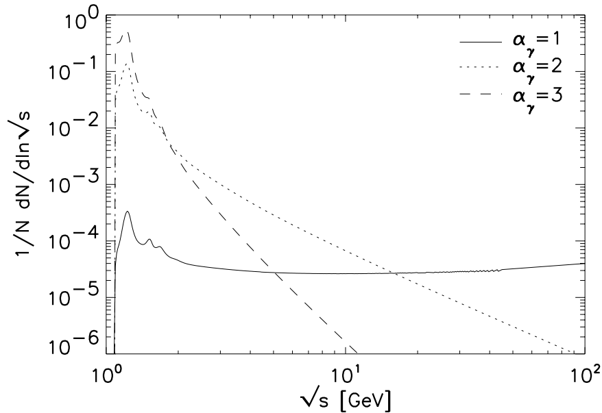
Figure 2 —Interaction probability distribution as function of the CMF energy with photon index \alpha_\gamma and proton spectrum n_E \sim E^{-2} .
