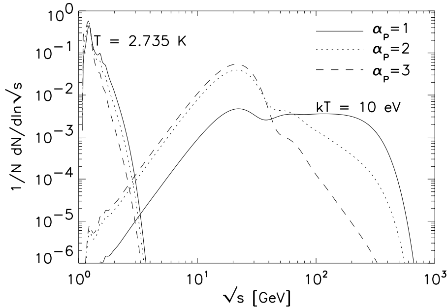
Figure 4 —Interaction probability distribution as a function of the CMF energy, for black body seed photon spectra and proton input spectra n_E \sim E_p^{-\alpha_p} in the energy range E_p = 10^6 - 10^{12} GeV.
