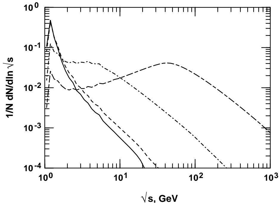
Figure 3 —Interaction probability distribution as a function of the CMF energy for a broken power-law seed photon spectra as observed in GRBs, using n_\epsilon \sim \epsilon^{-2/3} for 10^{-8} \text{ eV} \leq \epsilon \leq 1 \text{ keV} , and n_\epsilon \sim \epsilon^{-2} for 1 \text{ keV} \leq \epsilon \leq 100 \text{ keV} and proton spectrum n_E \sim E^{-2} with E_{\text{min}} \leq E \leq 10^{21} \text{ eV} and different minimum energies E_{\text{min}} = 10^{12} \text{ eV} (solid line), 10^{14} \text{ eV} (dashed line), 10^{16} \text{ eV} (dashed-dotted line) and 10^{18} \text{ eV} (dashed-dashed line). All quantities are in the fluid frame comoving with a small element of the blast wave region in GRB fireballs.
