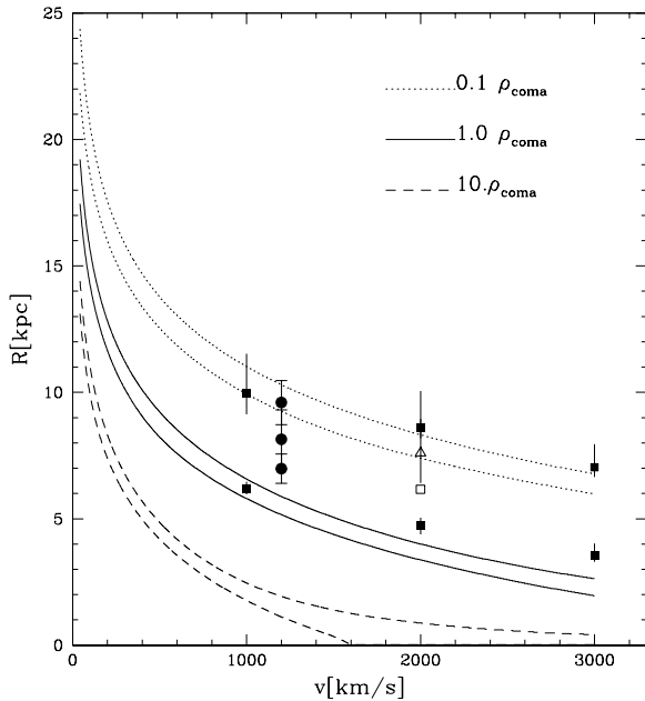
Figure 7. The size of the stripped gas disc, R_{\text{strip}} , as a function of the velocity flow for different cluster gas densities. The filled squares are from our simulations of face-on encounters, the open square and triangle are for edge-on and 45^\circ encounters.
