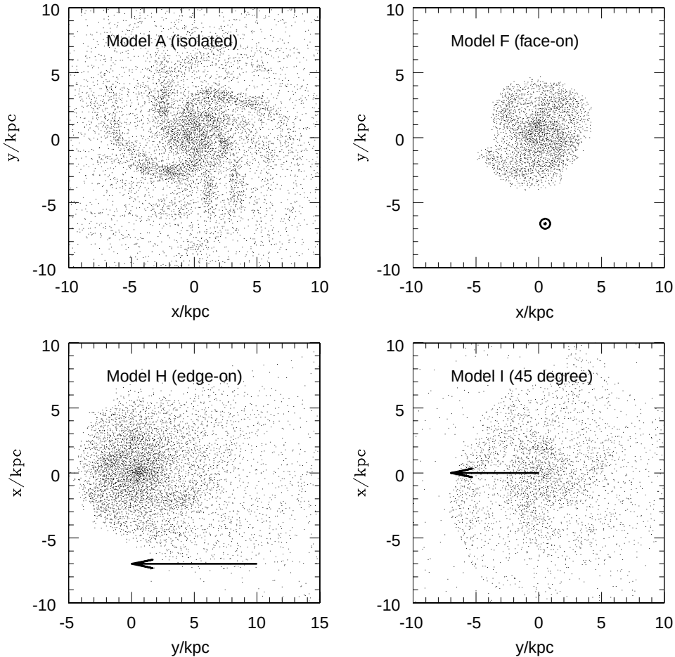
Figure 4. The positions of the gas particles plotted in the x - y plane (face-on) after \sim 10^8 yr of evolution. The arrows indicate the direction of motion (run A is the model in isolation).
