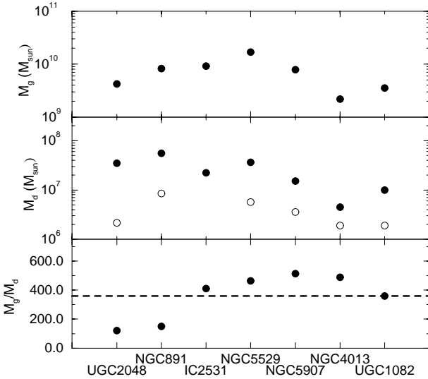
Fig. 11. The values of M_g (top graph), M_d (middle graph) and M_g/M_d (bottom graph) for each galaxy. All the masses are in units of M_\odot . For M_d we give a direct comparison between the values as calculated by our model (filled circles) and those calculated using the IRAS fluxes (open circles) wherever IRAS data were available. The dashed line in the last graph gives the mean value of the gas-to-dust mass ratio.
