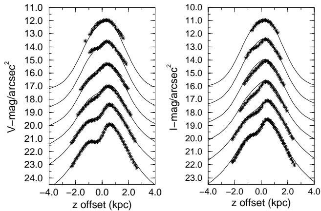
Fig. 6. Same as in Fig. 3, but for NGC 5529.
