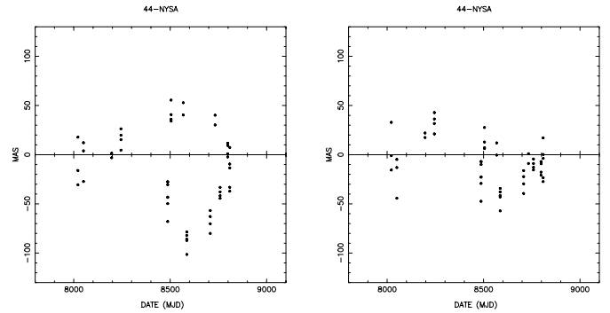
Fig. 2. Residuals of the observations of Nysa without any perturbation by Massalia ( left ) and assuming a value of 2.42 \cdot 10^{-12} M_\odot for its mass ( right ).
