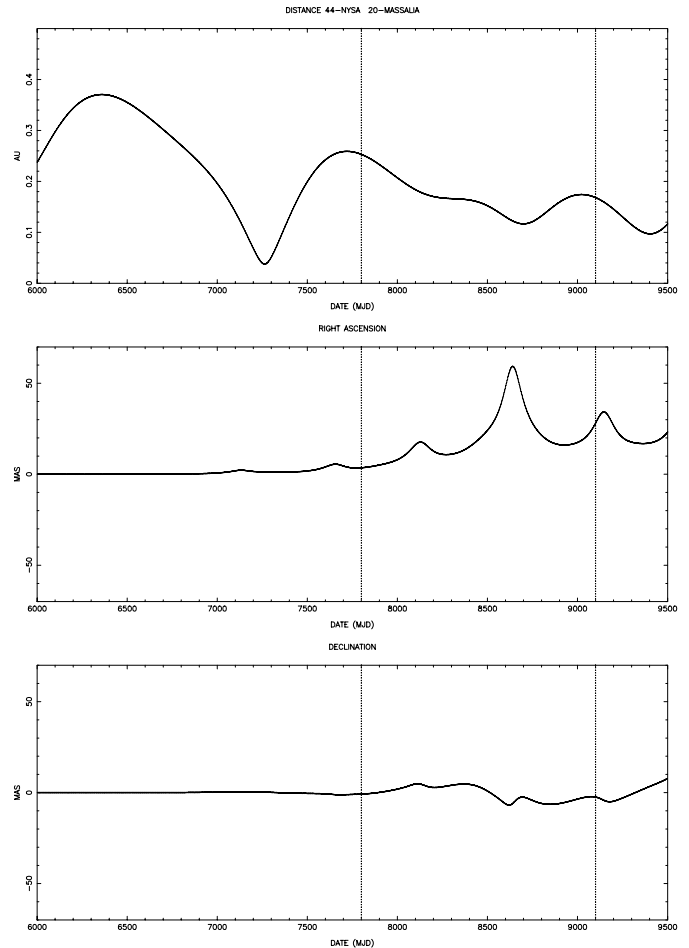
Fig. 1. Relative distance 20-Massalia 44-Nysa with respect to time (up, in AU) and differences in right ascension and declination between the perturbed orbit of 44-Nysa and the non perturbed one, assuming a value of 2.26 \cdot 10^{-12} M_\odot for the mass of Massalia (values in mas). The vertical lines give the beginning and the end of the Hipparcos mission.
