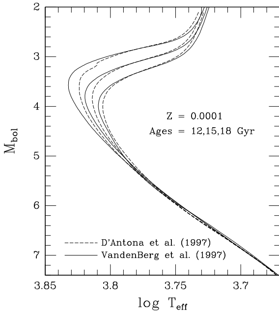
Fig. 6. Comparison of D'Antona et al. (1997) and Vandenberg et al. (1997) isochrones on the theoretical plane.
