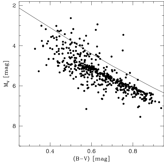
Fig. 3. Position of the sample objects of known [\text{Fe}/\text{H}] and \sigma_\pi/\pi < 20\% in the HR diagram using Hipparcos parallaxes, magnitudes and colours. The solid line is the Hyades main sequence.
