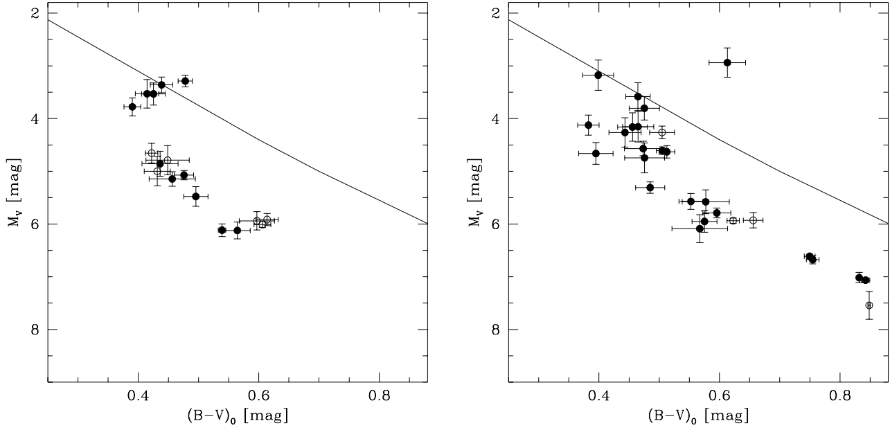
Fig. 4a and b. Position of the subdwarfs with \sigma_\pi/\pi < 15\% grouped into two [\text{Fe}/\text{H}] intervals: [\text{Fe}/\text{H}] < -1.8 colour-shifted to [\text{Fe}/\text{H}] = -2.2 (left), -1.8 < [\text{Fe}/\text{H}] < -1.2 colour-shifted to [\text{Fe}/\text{H}] = -1.5 (right). Detected or suspected binaries are indicated as open circles. The solid line is the Hyades main sequence.
