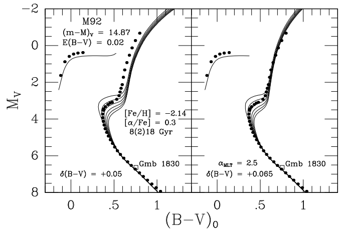
Fig. 8. Comparison of the M 92 sequence with Vandenberg (1997) model isochrones, for a higher value of the distance to M 92.
