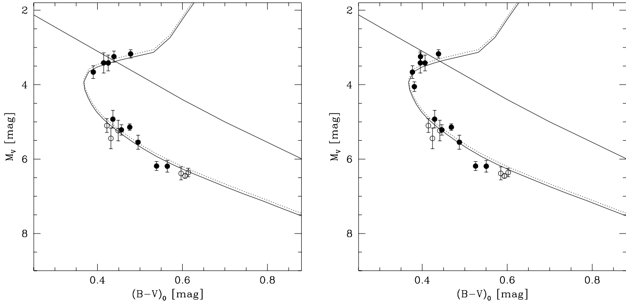
Fig. 5a and b. The fiducial sequence of M 92 fitted to the -2.6 < [\text{Fe}/\text{H}] < -1.8 subdwarfs, using the Coravel/CLL94 metallicity scale (left), and the scale of Axer et al. (right). Bias compensations and average binarity corrections to the absolute magnitude have been applied. The M 92 sequence is plotted with \mu_0 = 14.61 mag (solid line, fit with binaries corrected), and \mu_0 = 14.68 mag (dotted line, fit without including binaries). Suspected or detected binaries are shown as open circles. Colour-shifts \delta(B - V) have been applied towards a central [\text{Fe}/\text{H}] of -2.2 dex. The upper line is the Hyades main sequence.
