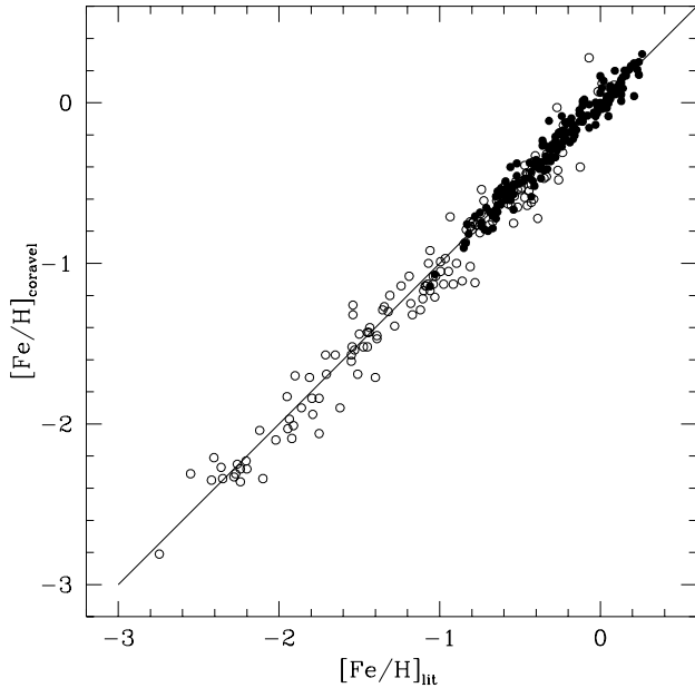
Fig. 2. [\text{Fe}/\text{H}]_{\text{Coravel}} vs. [\text{Fe}/\text{H}]_{\text{literature}} for the calibrators. The dispersion is 0.09 dex for the F-dwarfs from Edvardsson et al. (1993, filled circles), and 0.17 dex for the G dwarfs and subdwarfs from Carney et al. (1994, open circles).
