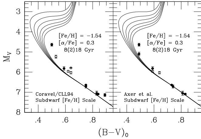
Fig. 9. Hipparcos subdwarfs with -1.8 < [\text{Fe}/\text{H}] < -1.1 dex, and \sigma_\pi/\pi < 5\% , colour shifted to [\text{Fe}/\text{H}] = -1.54 , compared with theoretical isochrones from Vandenberg et al. (1997), for the Coravel/CLL94 (left) and Axer et al. (right) metallicity scales. Detected or suspected binaries are shown as open circles.
