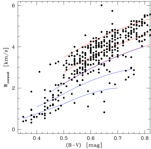
Fig. 1. The [\text{Fe}/\text{H}] calibration of the Coravel CCF equivalent width “W”. Lines of constant [\text{Fe}/\text{H}] are shown from [\text{Fe}/\text{H}] = -2 at 0.5 dex intervals, together with the location of the CLL94 calibrators.
