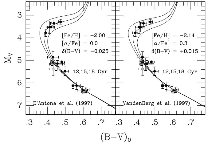
Fig. 10. Subdwarfs with -2.6 < [\text{Fe}/\text{H}] < -1.8 dex, shifted in colour to [\text{Fe}/\text{H}] = -2.2 , and isochrones for 12, 15, 18 Gyr from D'Antona et al. (1997) and Vandenberg et al. (1997). As noted, the isochrone colours were slightly adjusted in order to achieve the best possible fits to the unevolved subdwarfs. As the D'Antona et al. isochrones are for a scaled-solar mix of the heavy elements, isochrones for Z = 0.0002 ( [\text{Fe}/\text{H}] = -2.00 ) have been plotted to partially compensate for the neglect of an \alpha -element enhancement in these models. The mass-fraction abundance of all elements heavier than helium in the Vandenberg et al. computations is Z = 0.000254 .
