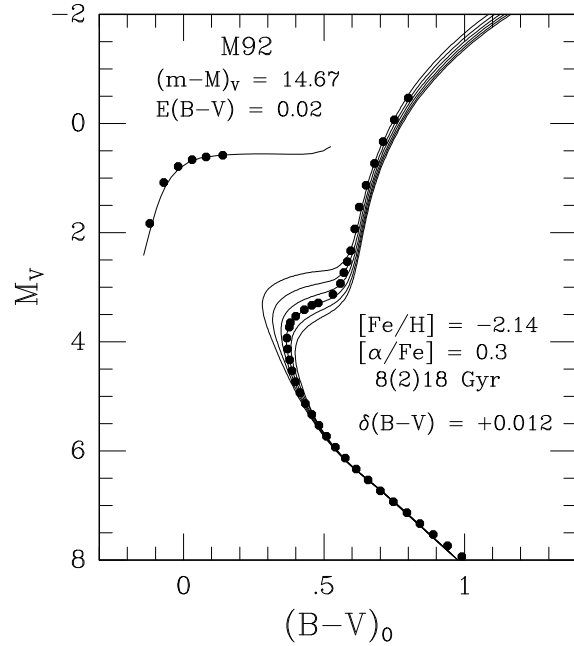
Fig. 7. Comparison of the M 92 sequence with Vandenberg et al. (1997) model isochrones, for the parameters shown.
