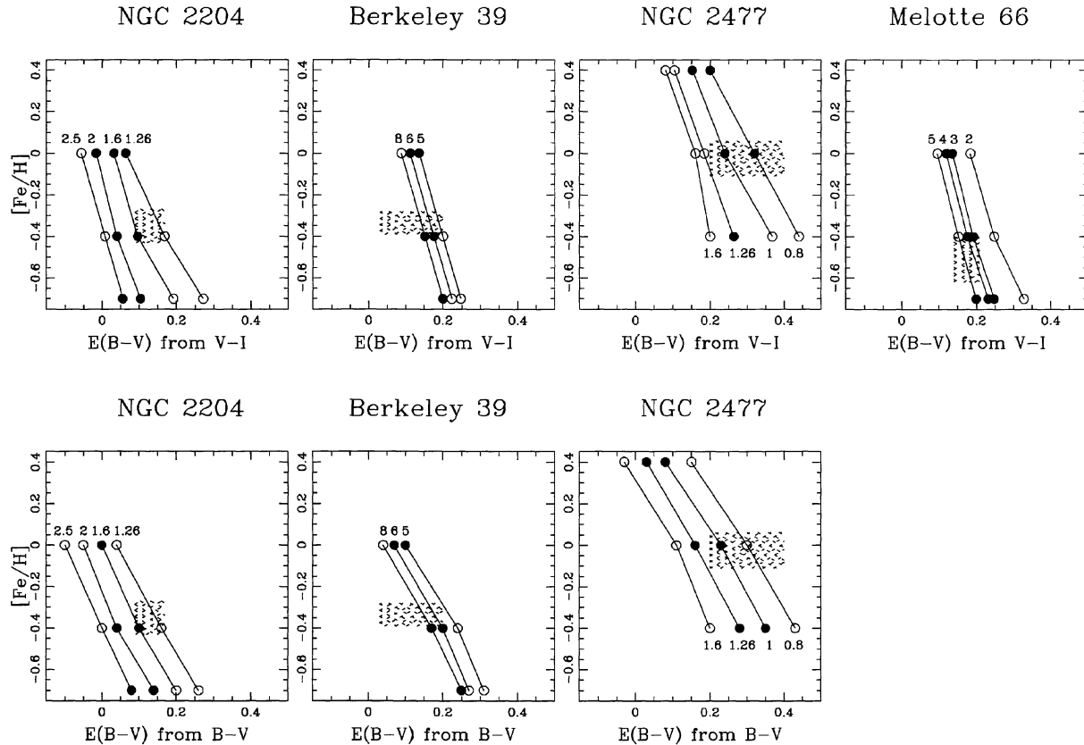
FIG. 4. For all the clusters in the sample, metallicities are plotted against reddenings determined from comparing isochrones at various ages. For three clusters, E(B-V) is determined from fits to both V-I and to B-V CMDs. Solid lines join the results from comparisons to isochrones of a given age, as labeled. Adopted metallicities and reddenings are represented as the hatched region in the grids, which show how well the models agree with these parameters.
