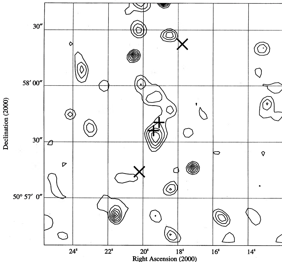
Figure 1. Contour map of the HRI image at the position of 3C 356. The X-ray image was binned in 2-arcsec pixels and smoothed. The crosses indicate the positions of the radio lobes and the pluses the positions of the two central optical/radio components, 3C 356N and S (see Fernini et al. 1993). None of the X-ray peaks represents a statistically significant excess above background at the 3\sigma level; there is an extended excess around 3C 356N significant at a level corresponding to 98 per cent confidence (see text).
