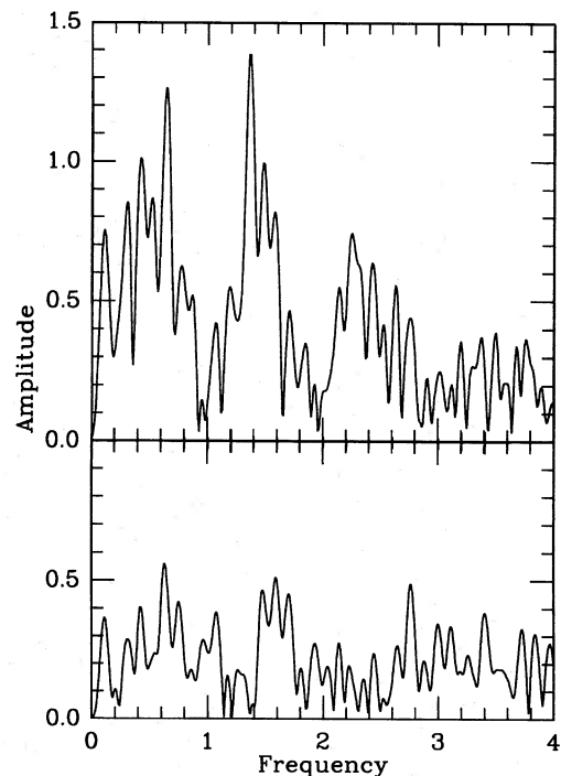
Figure 4. Periodogram of the radial velocities obtained by cross-correlation of the SAAO and MSSSO multi-order echelle data (top panel) and after removing the frequency f = 1.365 \text{ d}^{-1} (bottom panel). The amplitude is in \text{km s}^{-1} , the frequency in \text{cycle d}^{-1} .
