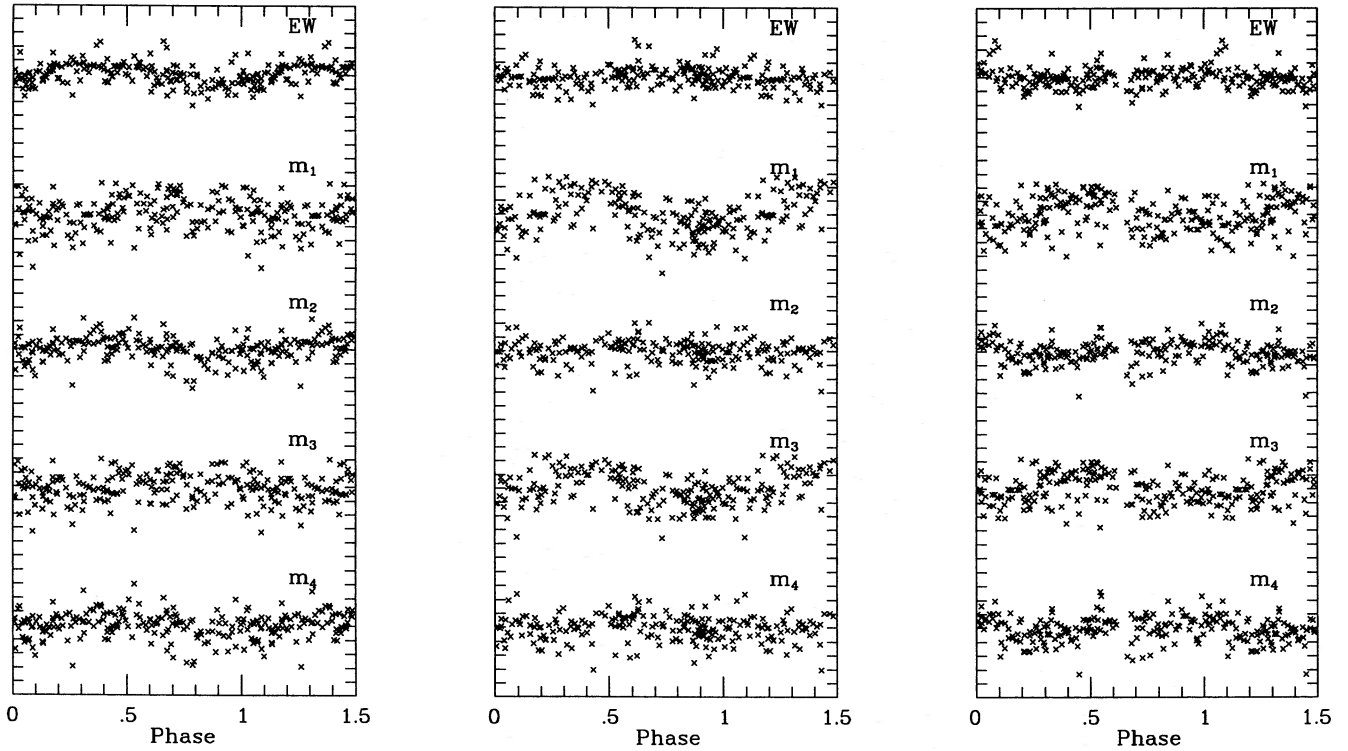
Figure 8. Phase variation of the equivalent width (EW) and the first four moments ( m_0 - m_4 ) of the Fe II line \lambda 5018.450 Å phased with f_1 (left), f_2 (middle) and f_4 (right). The epoch of phase zero is JD 244 9000. Tick marks are spaced at intervals of 0.02 Å for EW and 2 km s ^{-1} for m_1 . The other moments are plotted on an arbitrary scale.
