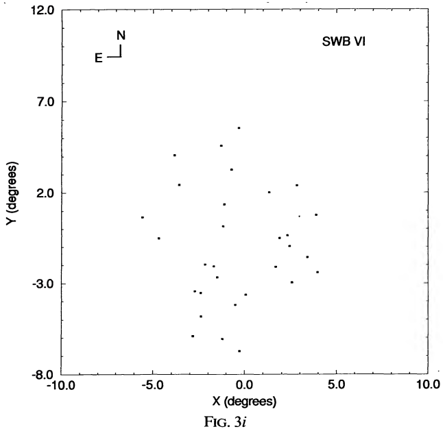
FIG. 3.—Spatial distributions: (a) whole sample, (b)–(j) age groups SWB 0 to SWB VII, respectively. NGC 1841 is outside the frame and is indicated by an arrow in (a) and (j).
