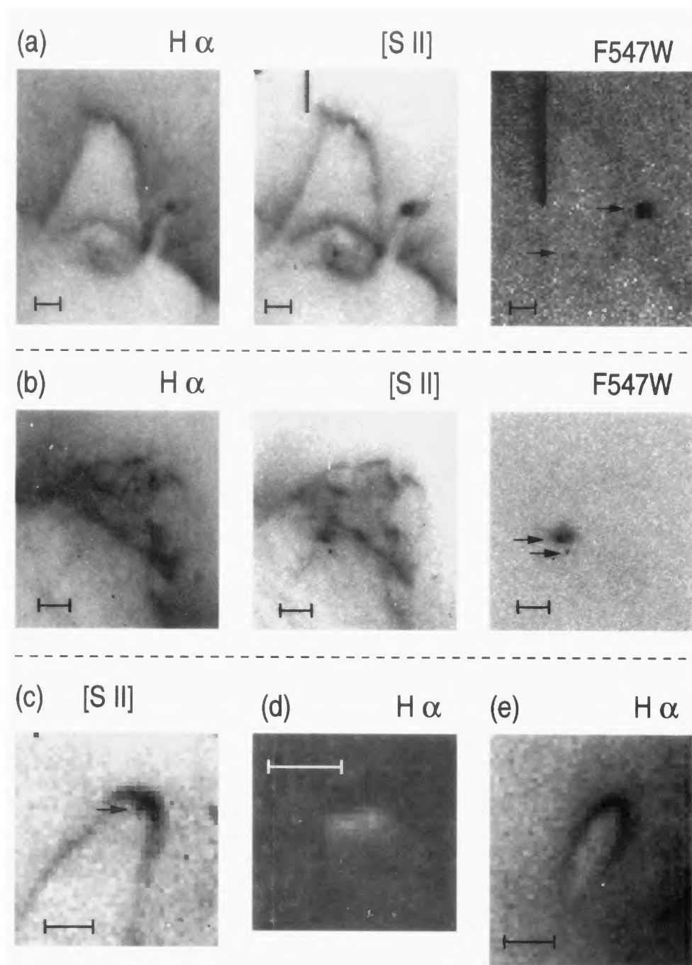
FIG. 10. Images of a few interesting structures in M16 which are associated with YSOs. The small tick in each image indicates 1'' = 3 \times 10^{16} cm, or 2000 AU. (a) H\alpha , [S II], and F547W images of two YSOs and their environments. The YSOs are indicated by the small arrows in the F547W frame. The right hand object (M16-E42) has been caught at the instant it is emerging from the globule from which it formed. This is a strong K-band object as well. Conversely, the object on the left appears to be located in a small cavity, possibly formed by its own wind. Also note the small globule (M16-E39) emerging near the top of the larger cometary structure (M16-E40) near the top of the field. (b) Structure at the head of column II, including a small, one-sided reflection nebula. On the basis of its morphology we believe this reflection nebula to be a disk and outflow cavity in the molecular cloud that are being uncovered by the photoevaporation front. The “blisters” at the head of column II appear to be a tight cluster of about 8 globules. This is a region of bright K-band emission. (c) An EGG in which the embedded star (indicated by the arrow) is just beginning to emerge. The star is also seen at K. (d) M16-E52 is an apparently disk-like structure. The faint emission near the center of the object is continuum emission, and may be reflection from an embedded YSO. (e) An isolated EGG (M16-E1) located just to the north of column I. This object is associated with a bright K-band source.
