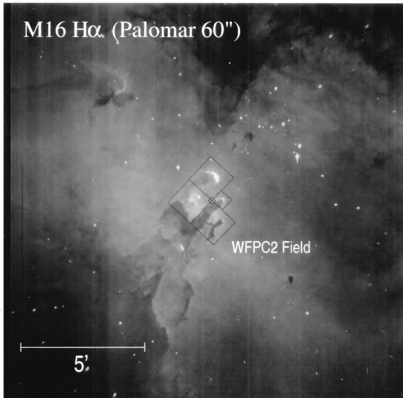
FIG. 1. Ground-based H \alpha image of M16 showing the field observed with WFPC2. North is at the top and east is to the left. The bar shows a length of 5' which is \sim 9 \times 10^{18} cm at a distance of \sim 2000 pc.
