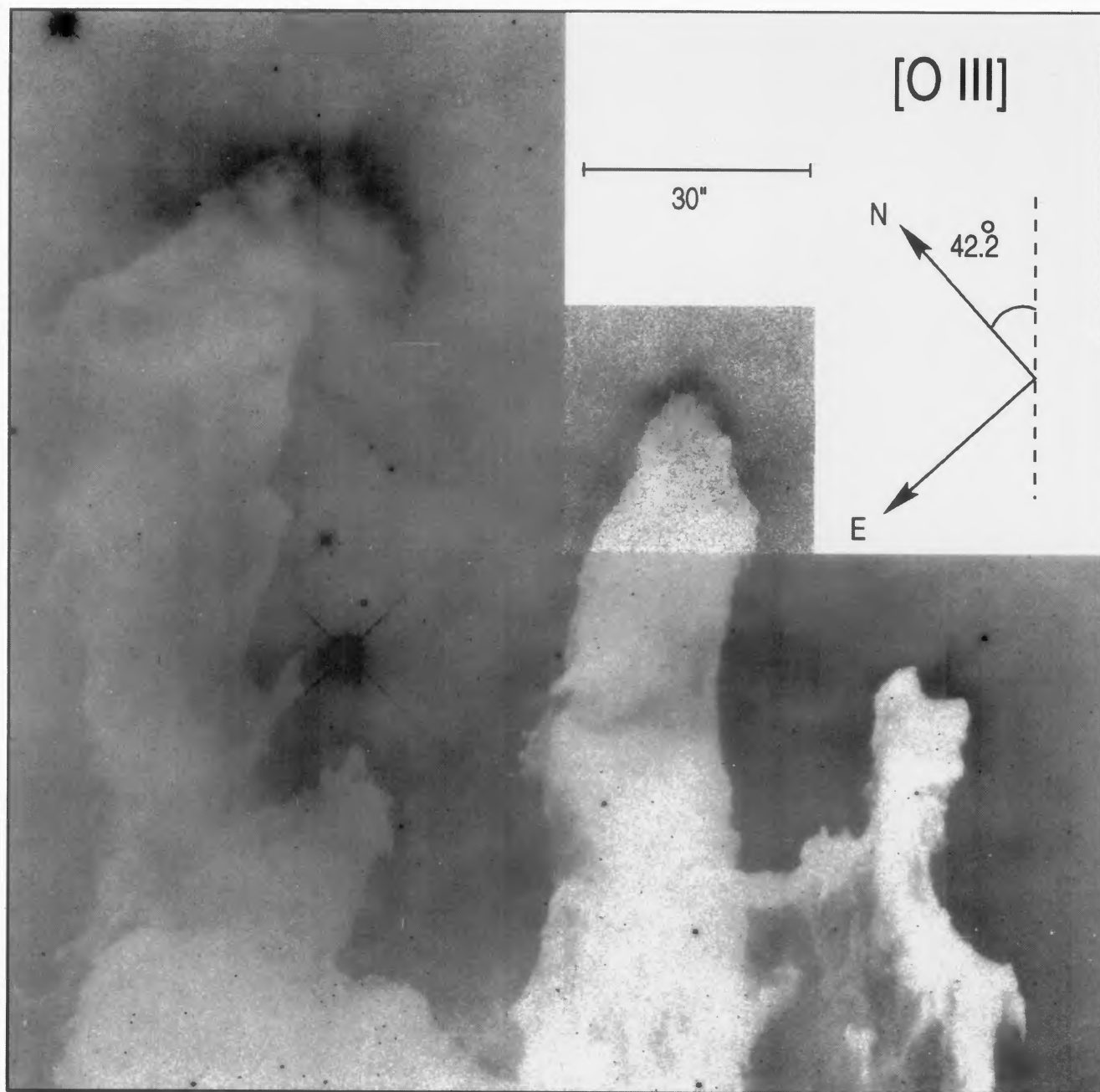
FIG. 4. WFPC2 image of elephant trunk structures in M16 taken through the F502N filter, which isolates light from [O\ III] \lambda 5007 . The display uses a square root stretch.
