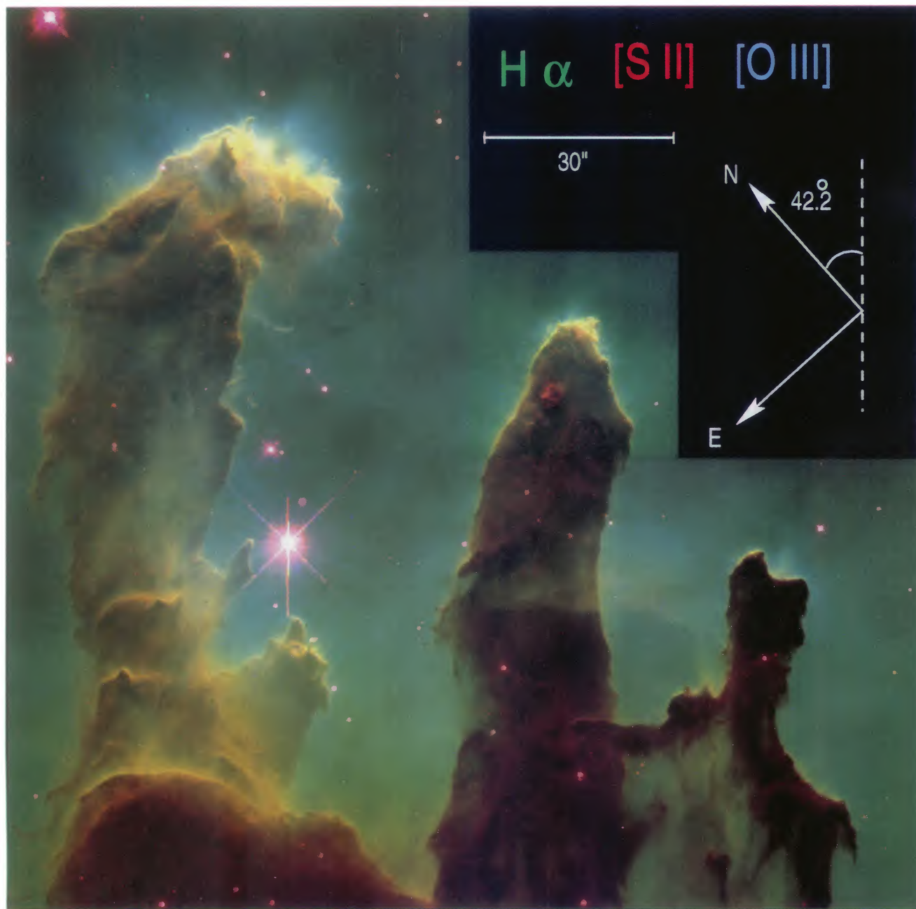
FIG. 5. Color composite of the WFPC2 images of M16. Red shows emission from [S\ II] . Green shows emission from H\alpha . Blue shows emission from [O\ III] .
