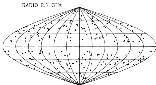
FIG. 5—The distribution of the 233 strongest 2.7 GHz extragalactic radio sources is shown in galactic coordinates. The data were obtained from Wall and Peacock (1985). These sources are associated with very distant galaxies, and they are apparently distributed isotropically and randomly in the sky. Sources in the ‘zone of avoidance’ close to the galactic equator are not shown to avoid confusion with the large number of galactic sources.
