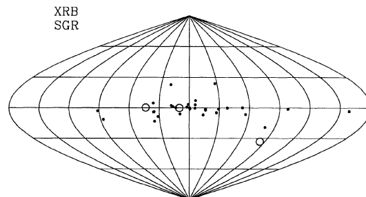
FIG. 6—The distribution of the galactic X-ray bursters (XRB—filled circles) and the three known soft gamma repeaters (SGR—open circles) is shown in galactic coordinates. The data were obtained from van Paradijs (1995 private communication). Notice the strong concentration of sources toward the galactic plane and the galactic center.
