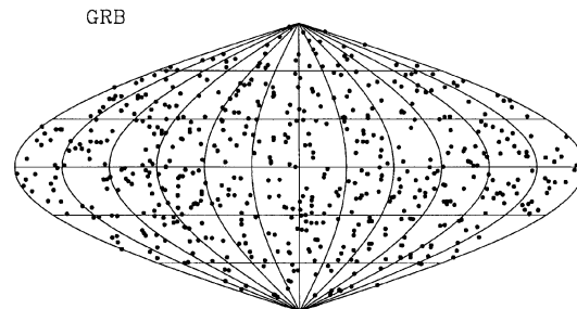
FIG. 7—The distribution of the 585 gamma-ray bursts (GRB) from the second BATSE catalog is shown in galactic coordinates. The data were obtained from GRNEWS at Goddard Space Flight Center. Notice the random and isotropic distribution of sources over the sky.
