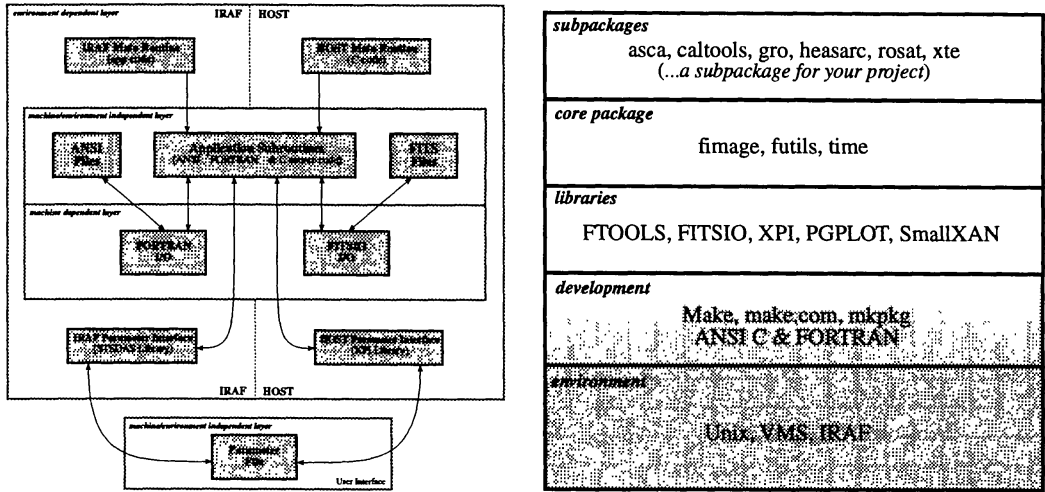
Figure 1. FTOOLS Task and Package Design.
