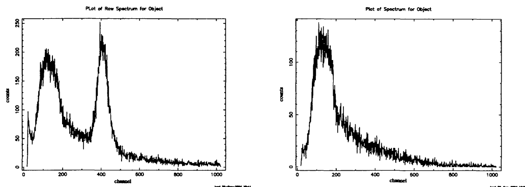
Figure 2. Raw spectrum on left showing supernova remnant with calibration source and the spatially filtered spectrum to right.
