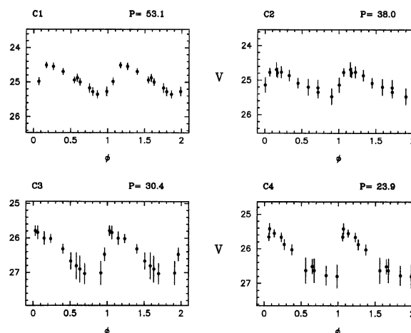
FIG. 18. V light curves for examples of Cepheids in M100, from Freedman et al. (1994b).
