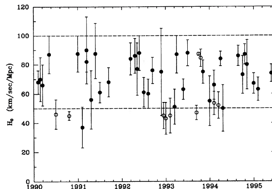
FIG. 6. Same as Fig. 5, but showing papers published since 1990. Open symbols denote papers published by de Vaucouleurs or Sandage and collaborators.
