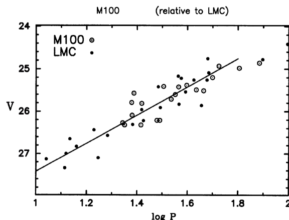
FIG. 19. Preliminary period–luminosity relation for Cepheids in M100, from Freedman et al. (1994b).
