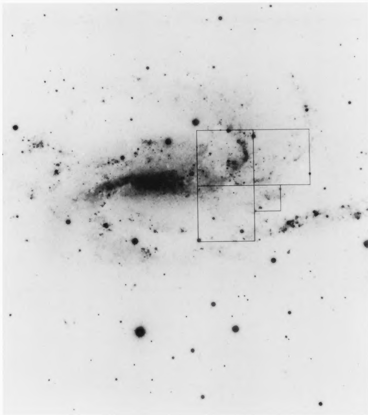
FIG. 15. Comparison of ground-based image of NGC 925 with median averaged WFPC2 exposure. The inset in the ground-based image shows the region observed with WFPC2 by Silberman et al. (1994).
