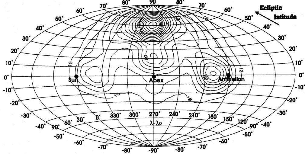
Figure 3. Activity contours for the combined Harvard radio surveys (a compilation of the Harvard I and Harvard II surveys). The abrupt ending of the contours near the edges of the projection is an artefact of the contour-smoothing method employed.
