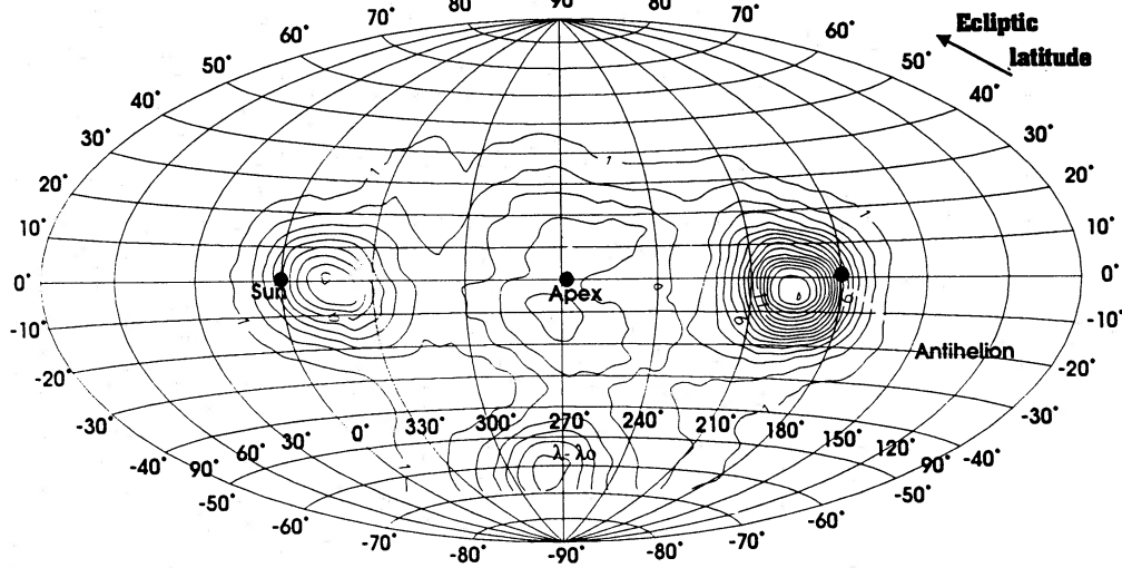
Figure 4. Activity contours for the combined Adelaide radio surveys (a compilation of the Adelaide I and Adelaide II surveys). See caption to Fig. 3 for details.
