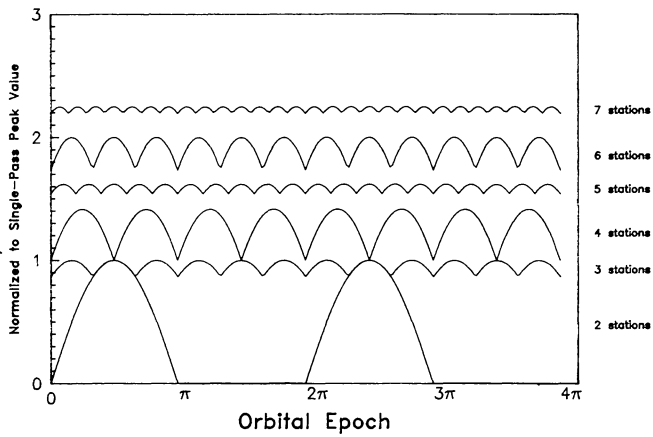
Fig. 2. The single-circuit steady-state gain available from a lossless planetary laser resonator is better for odd-sided, higher-order polygon geometries.
