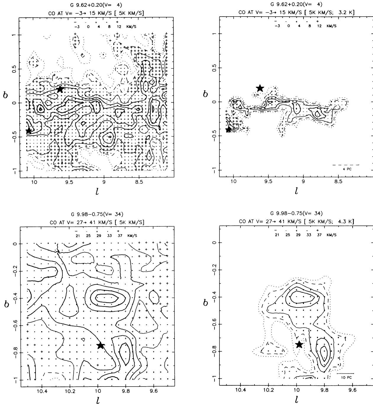
FIG. 13.—Maps of the integrated CO emission in the vicinity of 171 radio H II regions. For each group of associated H II regions two maps are shown: first, the integrated CO emission over a 15\text{--}20\text{ km s}^{-1} range centered close to the H II region position; second, the integrated CO emission including all (l, b, V) points above the boundary cutoff temperature T_c which are simply connected to the CO emission peak. The second map in each case serves to isolate the CO emission associated with the H II region from the background CO emission. The contours of integrated intensity are in units of 1, 2, 4, 6, ... times the number given in the caption at the top of each map. The cutoff temperature T_c is specified at the right of the caption at the top of the second map in each case. The plus, minus, and open circle symbols superposed on the contour maps on a 3' grid (the sampling interval for most of the CO survey) indicate the CO centroid velocity for emission within the range of integration specified in the caption. The stars indicate the locations of H II regions within 10\text{ km s}^{-1} of the CO centroid velocity, and the largest star is the position of the H II region specified in the caption. The H II regions outside the cloud boundary in a given map will generally be found in association with another cloud or within the mapped cloud if the cutoff temperature is lowered. The bar at the lower right in the second map in each case shows the linear scale for the assumed distance of the H II region. When this bar is dashed, the near-far distance ambiguity for the H II region has not been resolved and the near distance is assumed.
