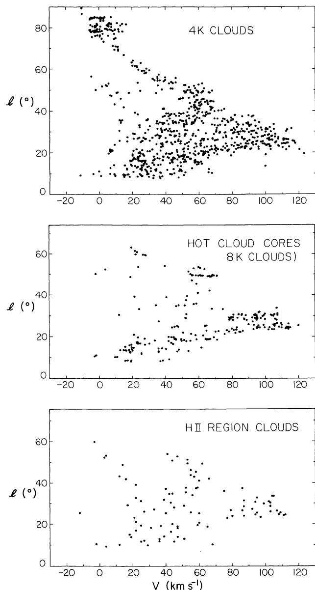
FIG. 3.—The (l, V) distribution of 4 K clouds, cloud cores, and H II region clouds is shown. The latter two samples exhibit tighter confinement in the (l, V) -plane, indicative of a spiral arm population.
