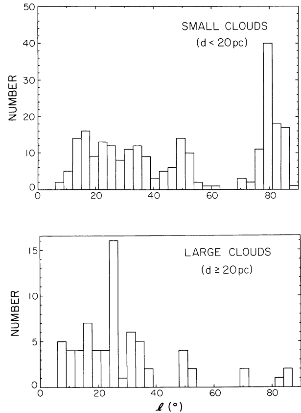
FIG. 6.—Longitude histogram for the large and small clouds from the 4 K sample (see Fig. 5).
