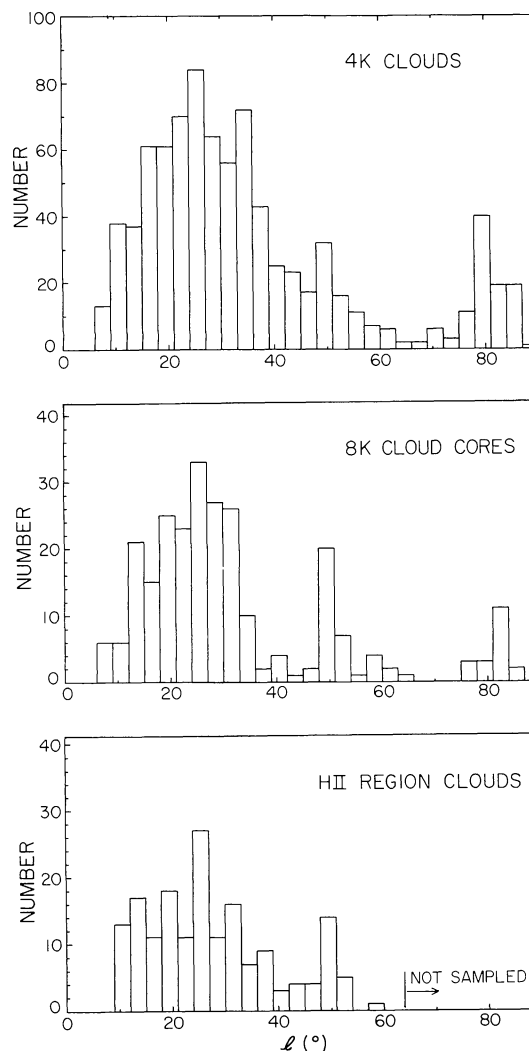
FIG. 4.—Histogram of the longitudes for the 4 K clouds, cloud cores, and H II region clouds. The latter two samples exhibit a marked deficiency in their number at l = 35^\circ – 45^\circ compared with the general cloud population.
