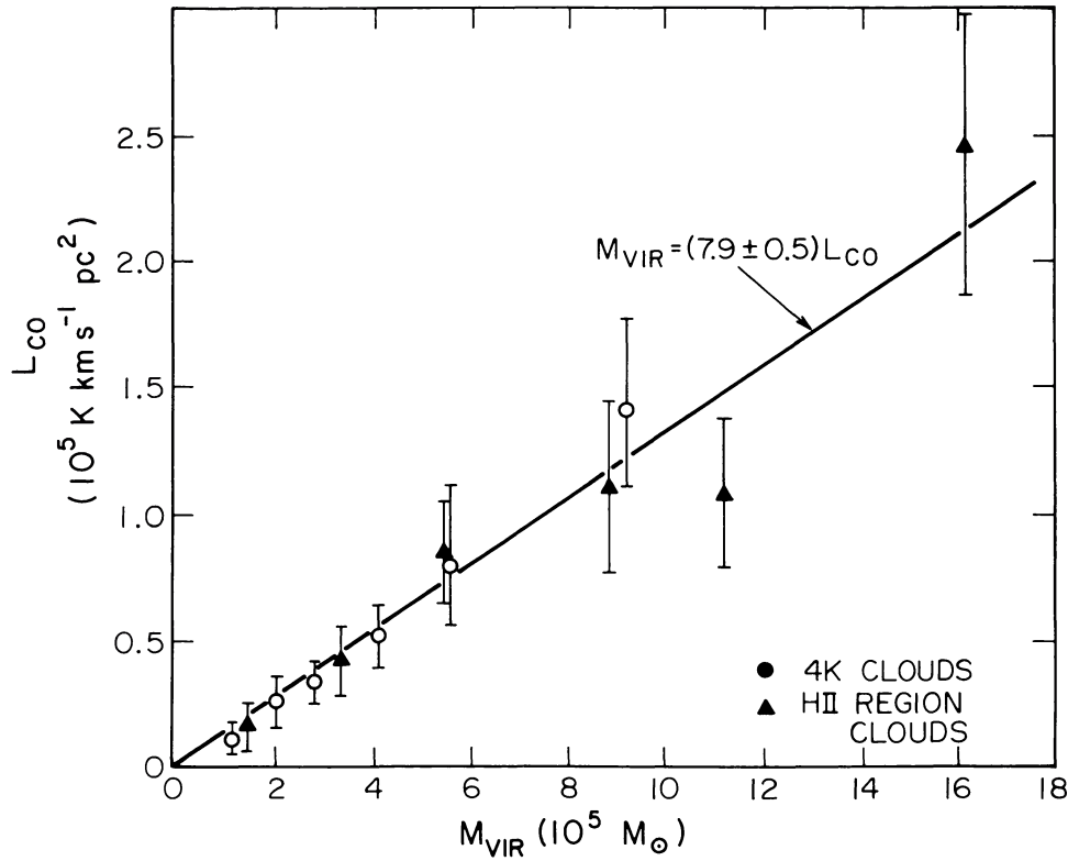
FIG. 7.—Variation of the CO luminosity L_{\text{CO}} ( \text{K km s}^{-1} \text{ pc}^2 ) integrated over the projected area of the clouds is shown as a function of the virial mass derived from the measured diameter and velocity dispersion. Only clouds for which the kinematic distance ambiguity is resolved are included in this sample. The straight line M_{\text{vir}} = (7.9 \pm 0.5) L_{\text{CO}} is fitted to the binned data over the range M_{\text{vir}} = 10^5 to 2 \times 10^6 M_{\odot} . The CO luminosity, velocity dispersion, and cloud sizes were measured at the same cutoff temperature in each cloud (col. [22] of Table 2).
