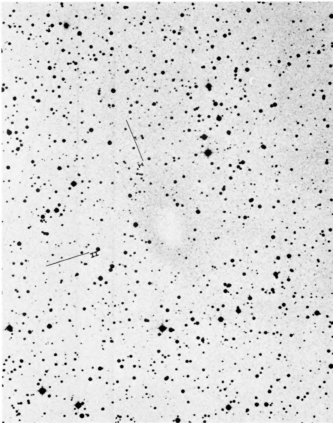
FIG. 1.—Enlargement of POSS O print showing the globule. Approximate central coordinates are \alpha(1950) = 0^{\text{h}}36^{\text{m}}17.0 , \delta(1950) = 52^{\circ}34'37'' (§ IIIa). Note the opaque inner core and bright diffuse rim. The cross marks above the globule image are 2' in length and denote the major and minor axis directions for the densitometric tracings in Fig. 2.
