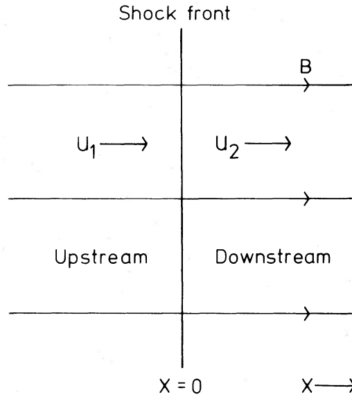
Figure 1. A parallel shock viewed in the frame in which it is stationary.
