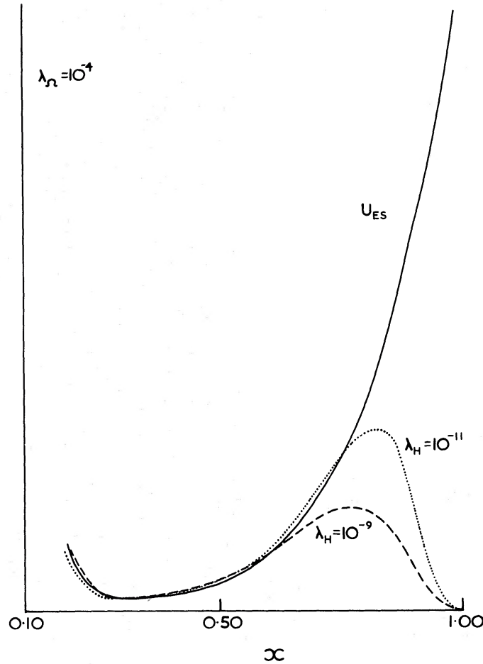
Figure 3. \lambda_\Omega = 10^{-4} , even parity fields. The curve labelled U_{ES} gives the radial component of the Eddington–Sweet velocity field along the axis of the star, the curves labelled with values of \lambda_H give the axial radial components of the computed circulations.
