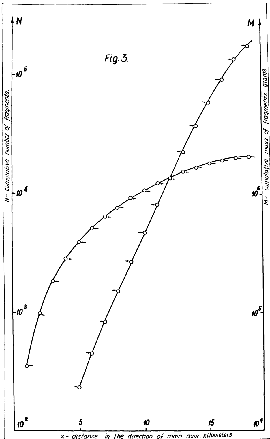
Fig. 3 The cumulative number N and the cumulative mass M (grams) of fragments from Pułtusk meteorite shower 1868 as dependent upon the upper limit of integration.
