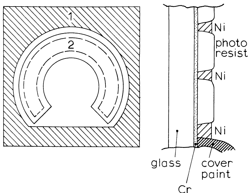
Fig. 5. Final stage of the producing of a zone plate (2) Within a reinforced holding sheet (1).
