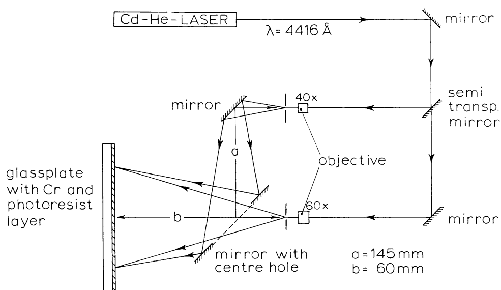
Fig. 3. Optical arrangement for the production of zone plates with a split-up laser beam.
