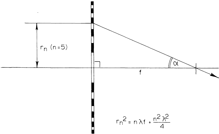
Fig. 1. Image formation conditions for a zone plate.
