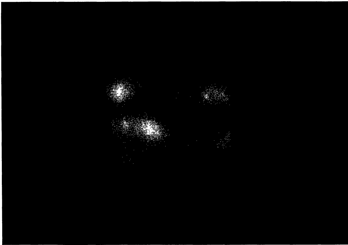
Fig. 2. Image of the sun in 51 Å radiation obtained with a non-apodised zone plate camera on October 3, 1967. Original image diameter 4 mm.
