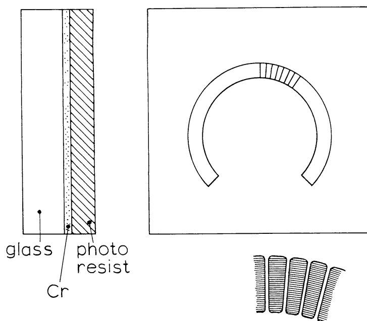
Fig. 4. First stage of the production of a zone plate.
