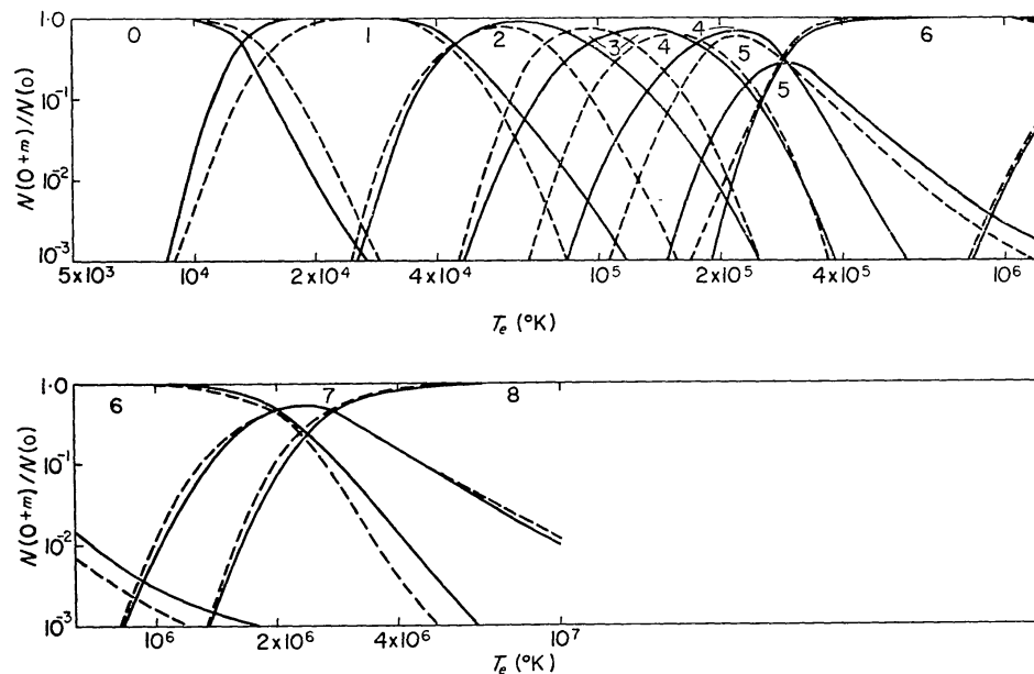
FIG. 1. The ionization equilibrium of O ions. The full lines illustrate the present calculations which are applicable to the Sun. The dashed lines show the results of House (1964).
