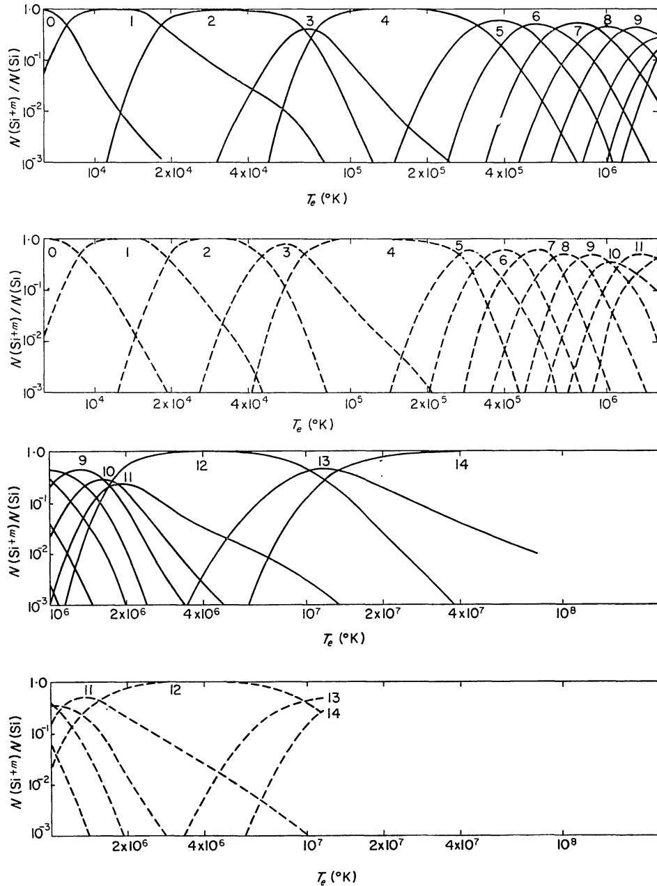
FIG. 2. The ionization equilibrium of Si ions.
