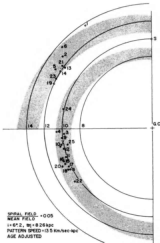
FIG. 7.—Places of formation of stars as determined with the inclusion of a spiral gravitational field travelling at a pattern speed of 13.5\text{ km sec}^{-1}\text{ kpc}^{-1} and having an intensity equal to 5 per cent of that of the symmetrical gravitational field.
